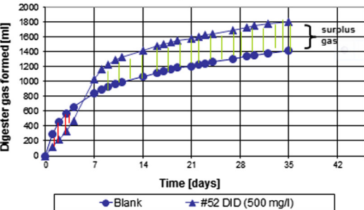
Anaerobic degradation test according to DIN 38414, part 8
