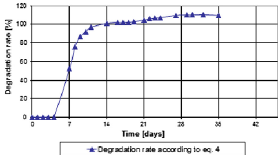
Quantification of degradation rate #52 DID (500 mg/l)
