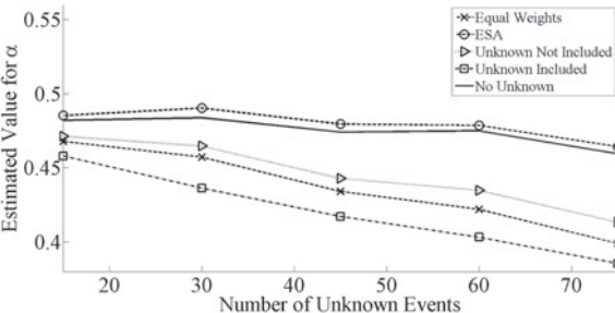
Estimates for \alpha , True \alpha = 0.5
