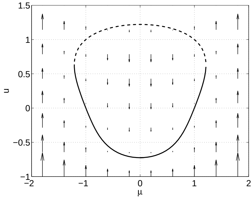
FIGURE 1. Dynamics of (2). The curve of stable fixed points is shown solid, while the unstable fixed points are shown dashed. Arrows show the direction of solutions for fixed \mu .
