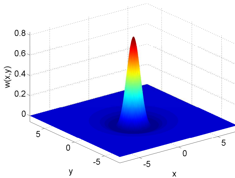
FIGURE 8. The Mexican-hat coupling function (33).
