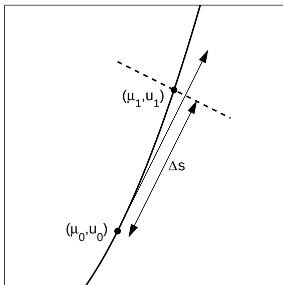
FIGURE 2. A schematic showing the relationship expressed by (3). The curve of solutions is solid, and the tangent to this curve at (\mu_0, u_0) is shown by the single-headed arrow. The dashed line is at right angles to this tangent.
