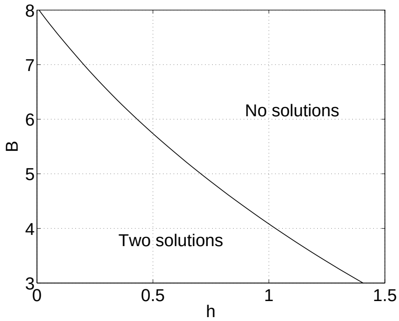
FIGURE 11. Curve of saddle-node bifurcations of stationary single-bump solutions of (10), where the coupling function is (57). A stable and unstable pair exist to the left of this curve. Fig. 4(a) is a horizontal “slice” through this figure at B = 6 . Parameters: N = 15, \beta = 20 .
