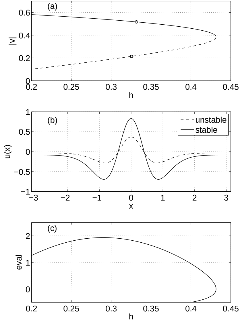
FIGURE 4. (a): Solutions of (19). The norm of v is plotted vertically; solid curve indicates stable solutions, dashed unstable. (b): Even solutions of (13) at the two points indicated in panel (a). (c): Most positive eigenvalue associated with solutions of (19). Parameters: N = 15, \beta = 20 .
