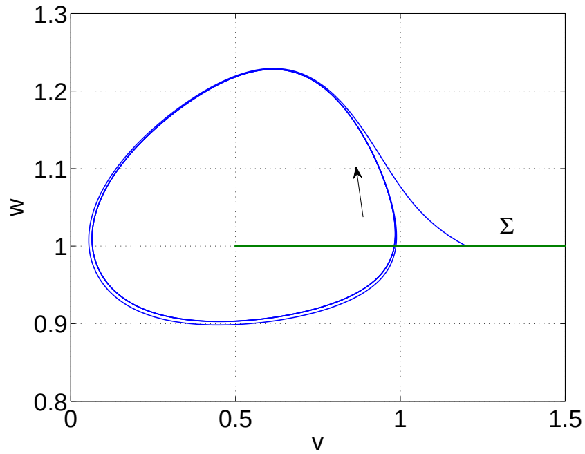
FIGURE 12. Finding a periodic orbit of (66)-(67) using a Poincaré section, \Sigma . The arrow indicates the direction of motion. See text for details.
