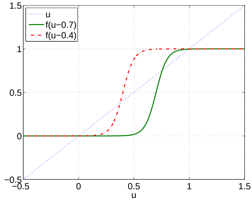
FIGURE 5. Solutions of (26) occur when the function f(u - h) intersects the diagonal, where f is given by (11) and \beta = 20 .
