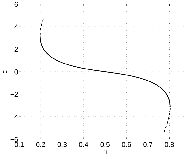
FIGURE 7. Speed of a front, c , as a function of h . Solid: stable, dashed: unstable. Parameters: \beta = 20 .
