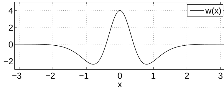
FIGURE 3. The connectivity function w(x) = 10 \exp(-4x^2) - 6 \exp(-x^2) .
