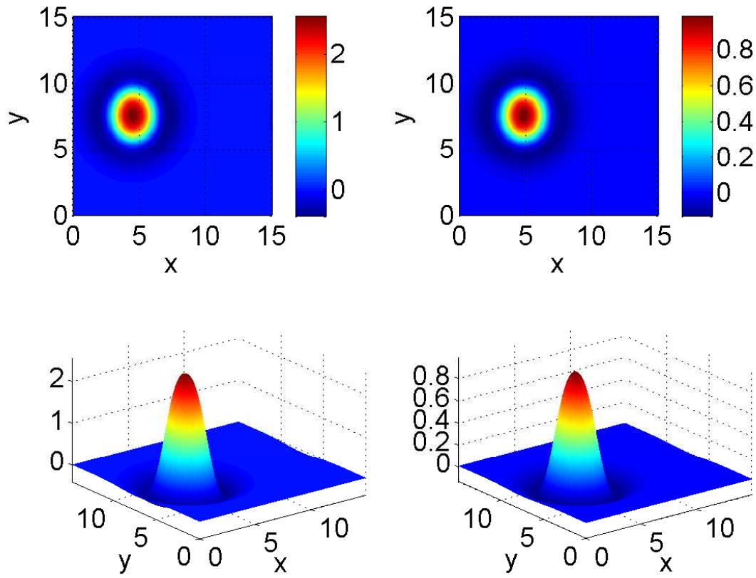
FIGURE 9. Leftward-moving bump solutions of (31)-(32). Left column: u , right column: a . Parameters: L = 15 , A = 2 , \beta = 5 , h = 0.8 , B = 0.4 , \tau = 3 .
