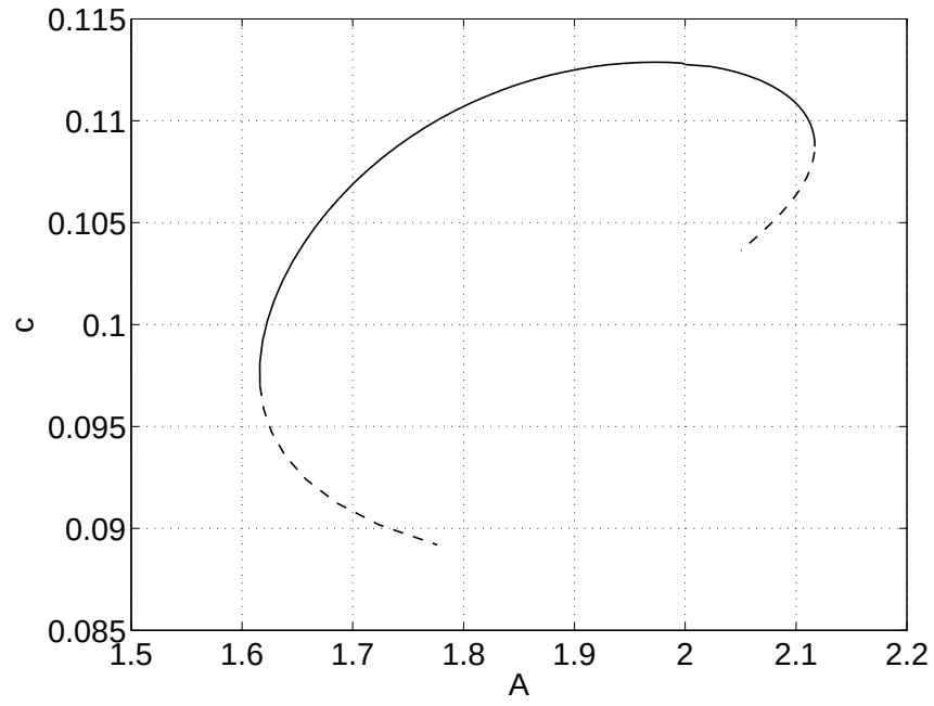
FIGURE 10. Speed of a two-dimensional bump, c , as a function of A . Solid: stable, dashed: unstable. Parameters: L = 15, \beta = 5, h = 0.8, B = 0.4, \tau = 3, N = 256 .
