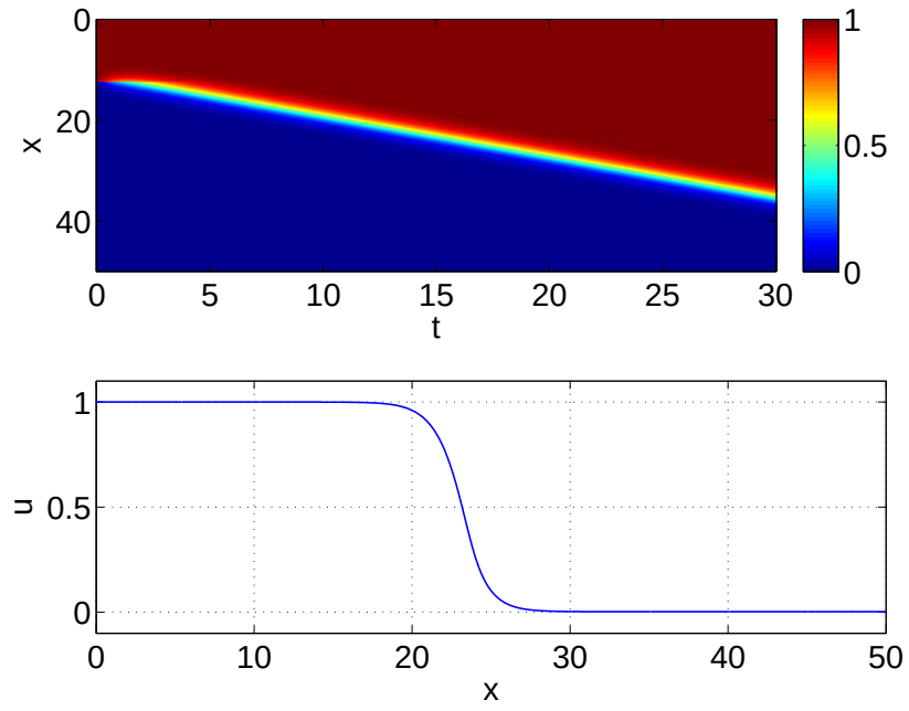
FIGURE 6. Top: space-time plot of a solution of (24)-(25), where the domain has been truncated to [0, 50] . Colour indicates the value of u . Bottom: front at t = 15 . Parameters: \beta = 20, h = 0.3 .
