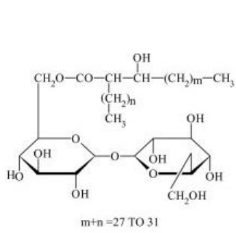
Trehalose monomycolates
