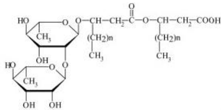
Dirhamnolipid
