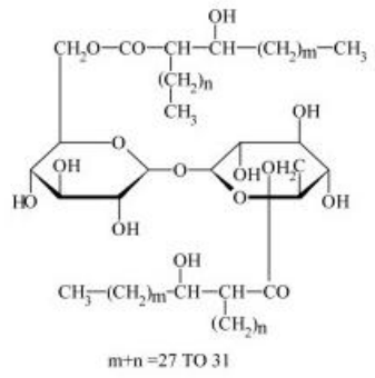
Trehalose dimycolates
