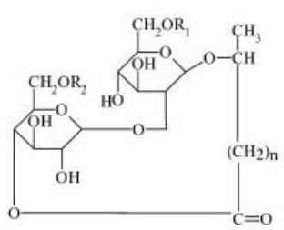
Lactonic Sophorolipid
