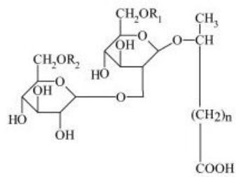
Acidic Sophorolipid
