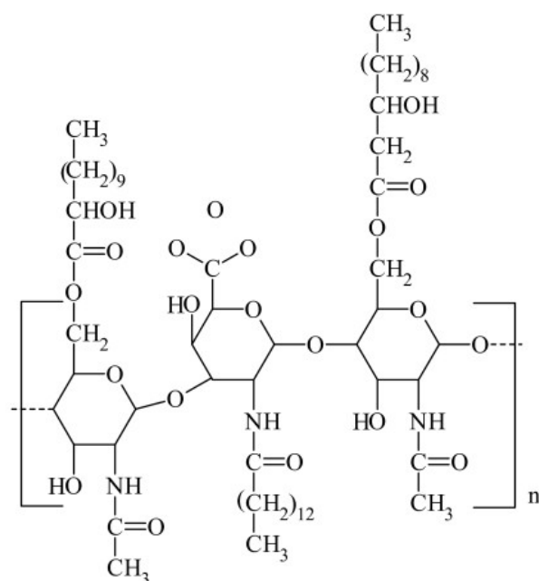
Emulsan
