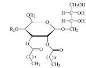
Mannosylerythritol lipids
