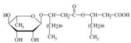
Monorhamnolipids
