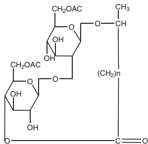
Lactonic Sophorolipid
