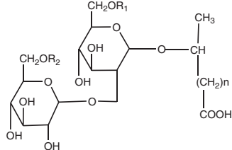
Acidic Sophorolipid
