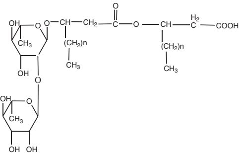
Dirhamnolipid
