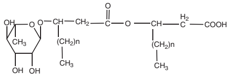
Monorhamnolipid
