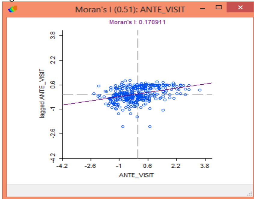
Figure 2- Moran's I Statistic
