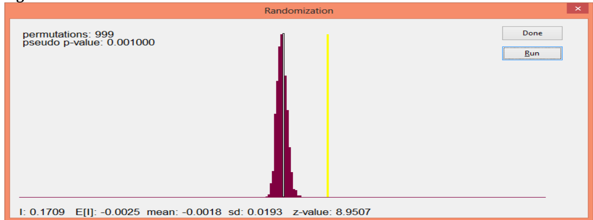
Figure 3- Inference for Moran's I statistic
