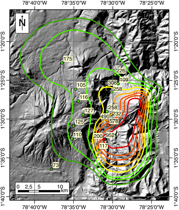
Tungurahua ash fallout (period 28/11 to 07/12/2011)
