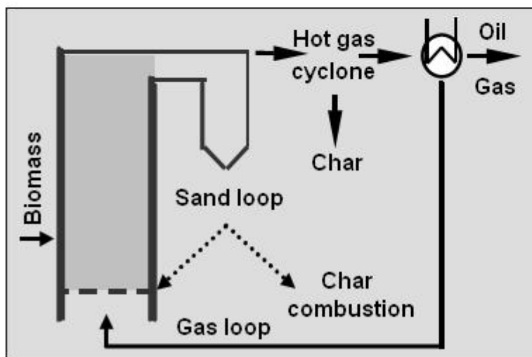
Circulated fluidized bed
