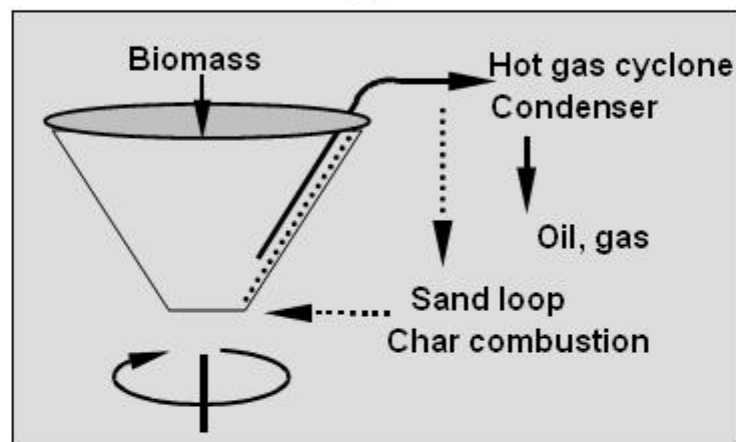
Rotating cone
