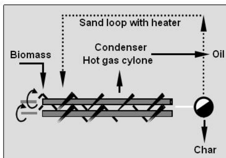
Twin screw mixer reactor
