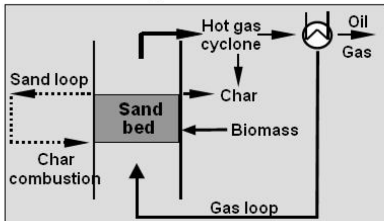
Bubbling fluidized bed
