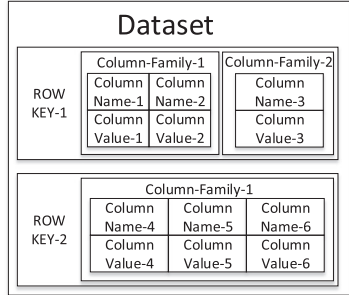
Column-Family Store
