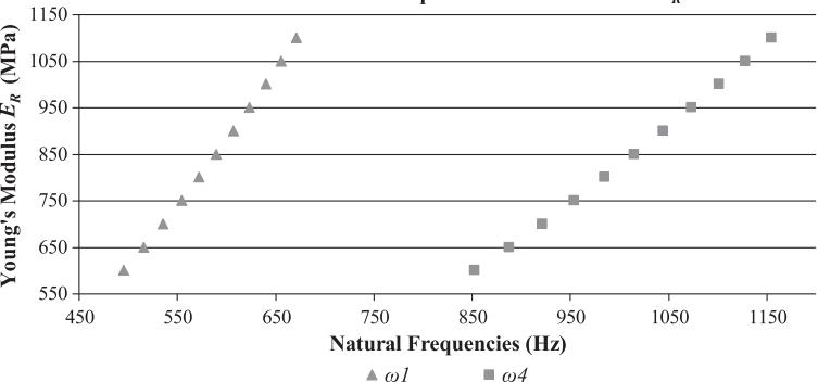
1 st and 4 th Natural Frequencies as a Function of E_R
