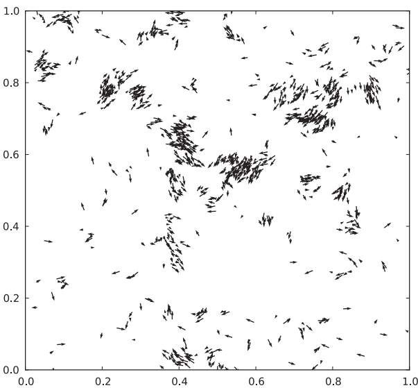
(c) High intermediate driving noise. \eta = 0.98
