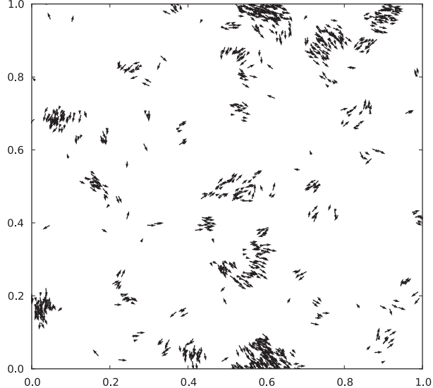
(b) Low intermediate driving noise. \eta = 0.785
