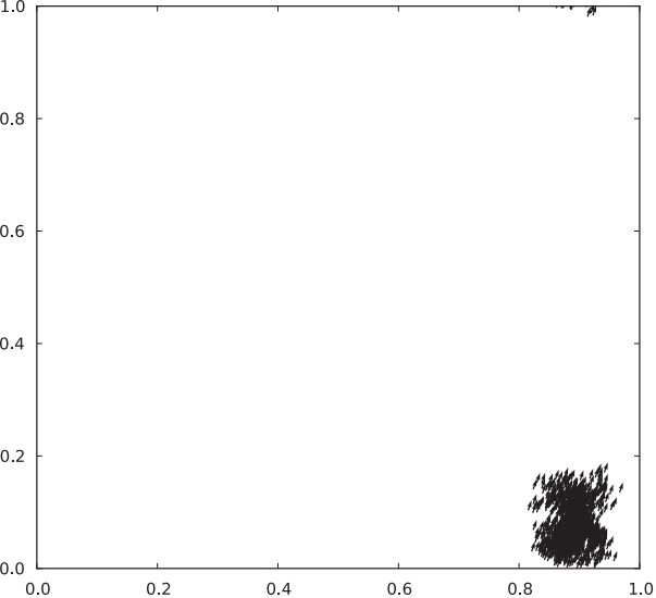
(a) Low driving noise. \eta = 0
