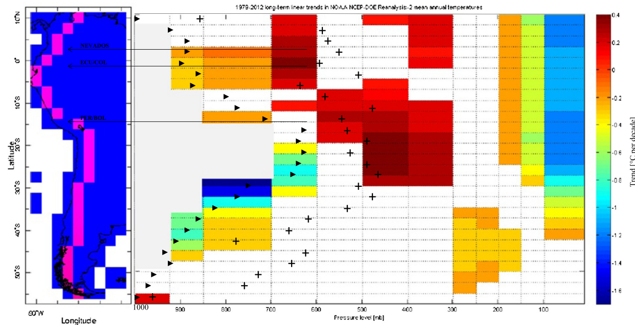
1979-2012 long-term linear trends in NOAA NCEP-DOE Reanalysis:2 mean annual temperatures
