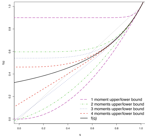
(b) Truncated Geometric distribution
