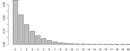
(b) Truncated Geometric distribution
