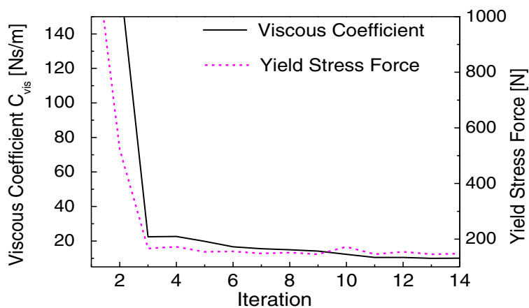
(b) viscous coefficient and yield stress force
