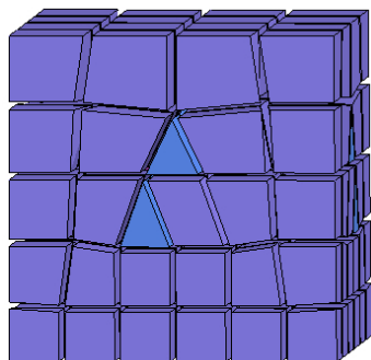
(5) mixed hexahedral mesh generated by Yamakawa-Shimada's algorithm (it contains 163 elements, of which 123 are hexahedra)
