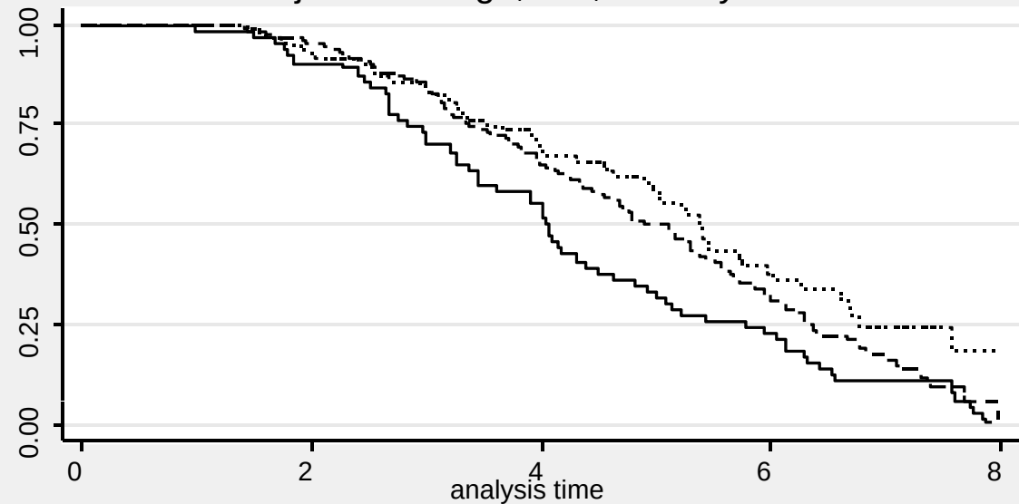
Survivor functions adjusted for age, sex, severity
