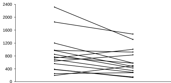
CKS2 (204170)
