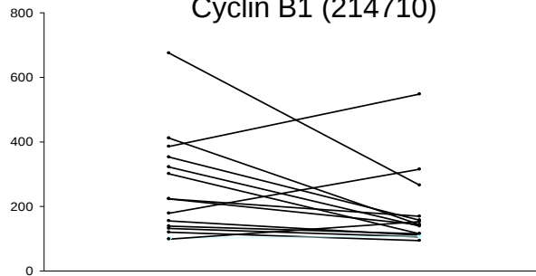
Cyclin B1 (214710)
