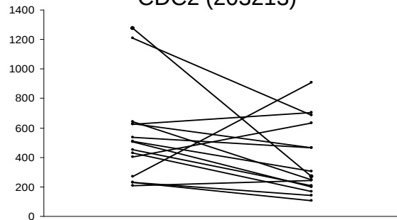
CDC2 (203213)
