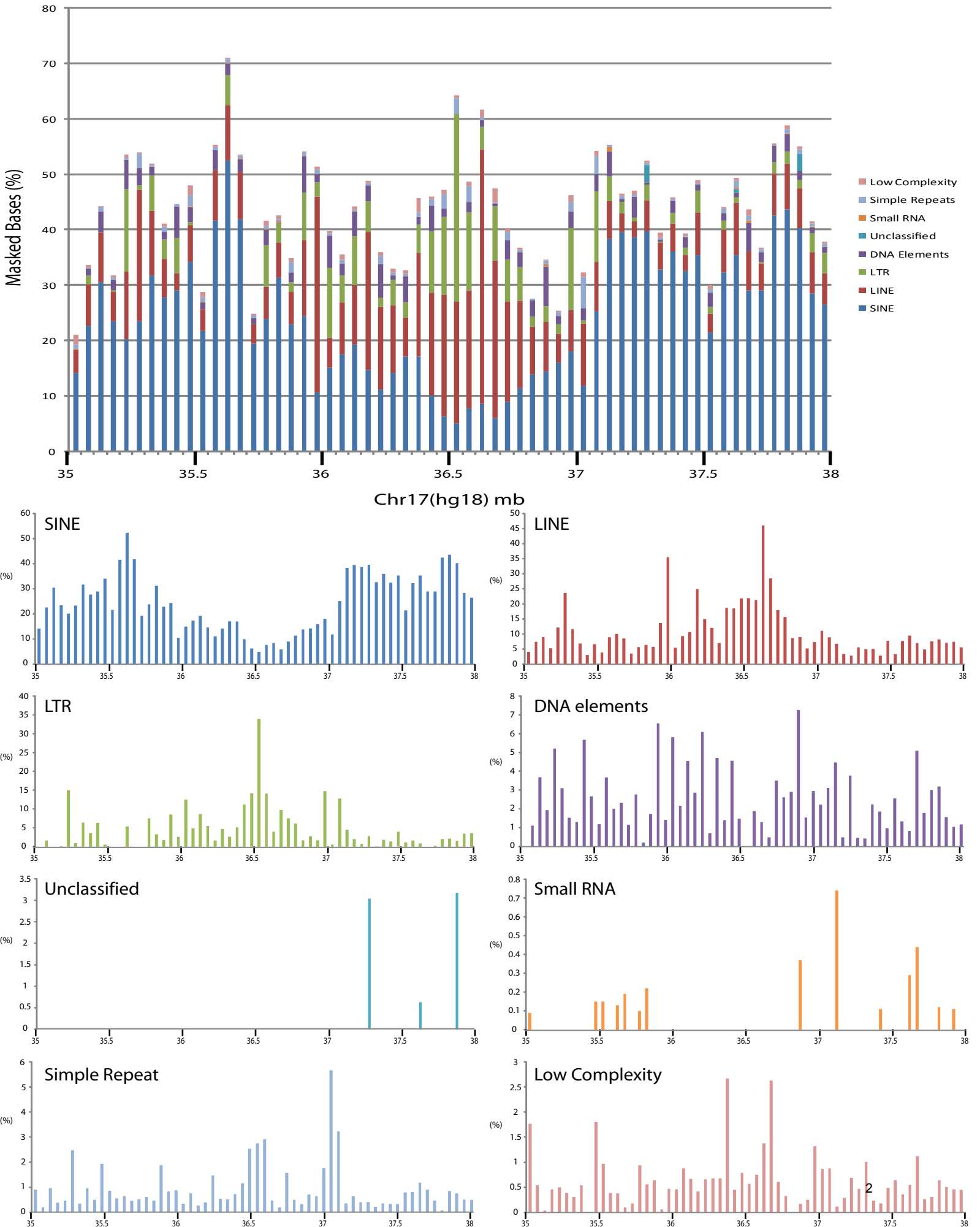
Figure S1. Repeat Masker Chr17 35-38Mb
