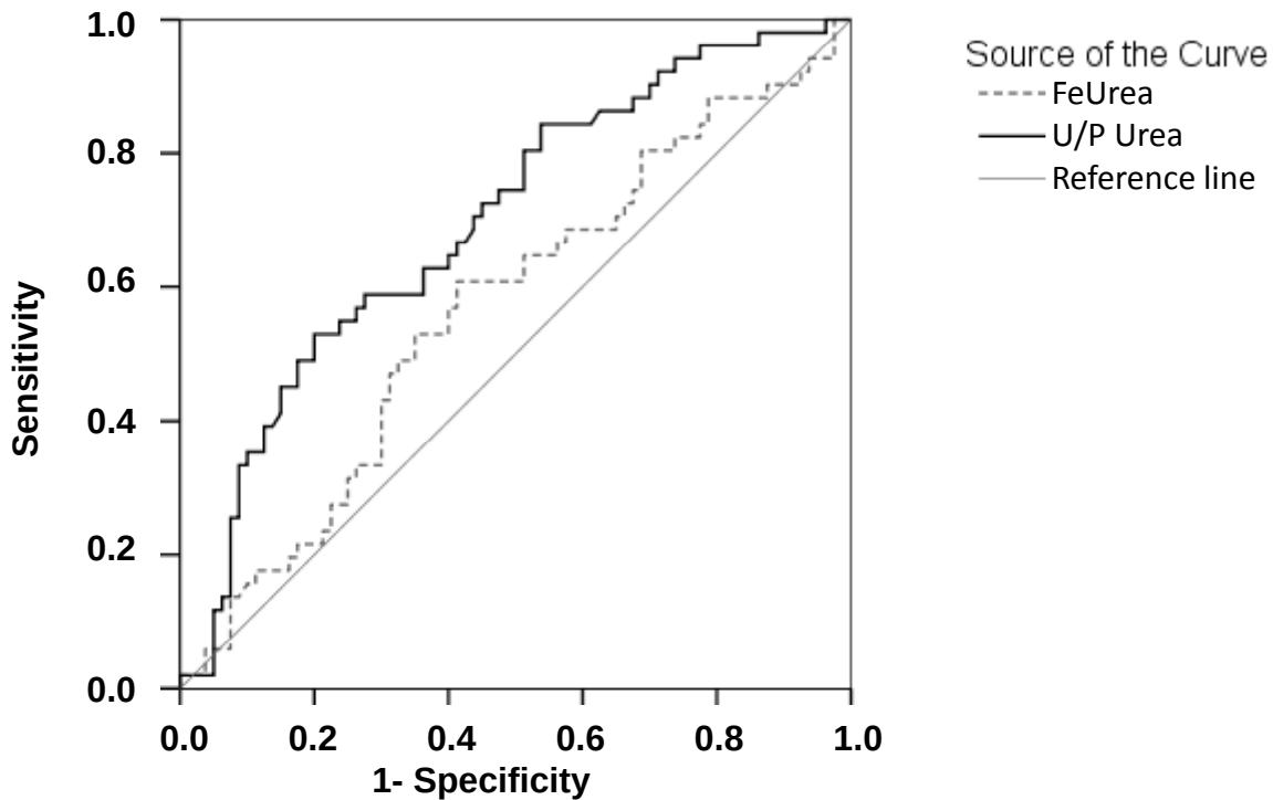
ROC Curve
