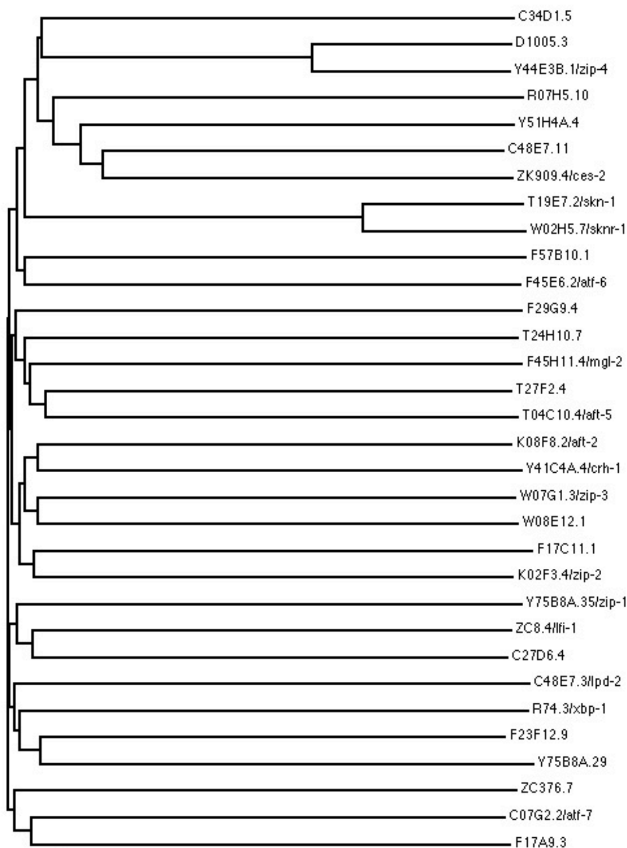
The bZIP family
