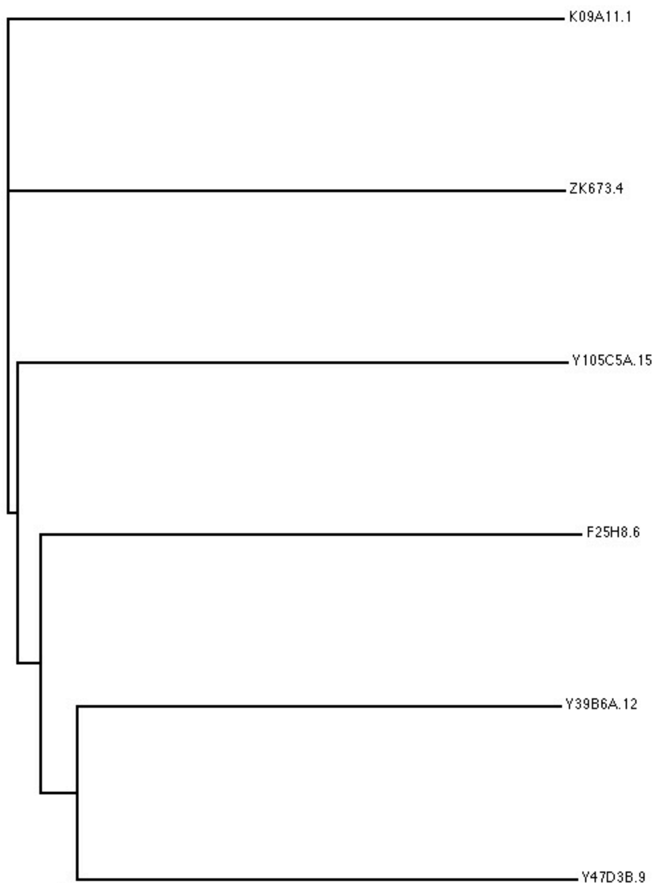
The BED Zinc Finger family
