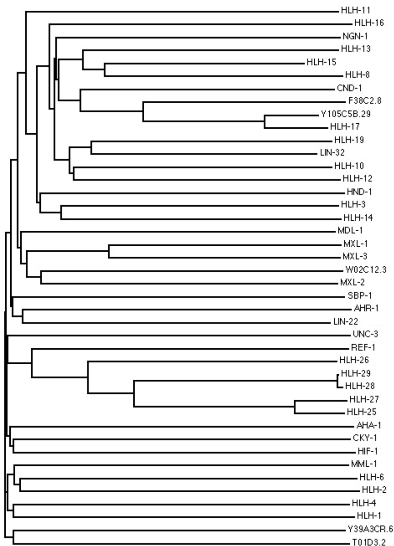
The bHLH domain family
