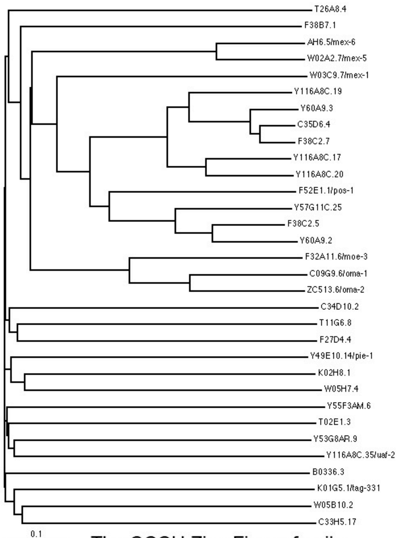
The CCCH Zinc Finger family
