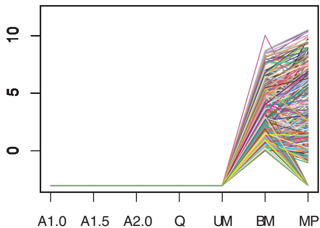
(e) Binucleate microspore peak N=662
