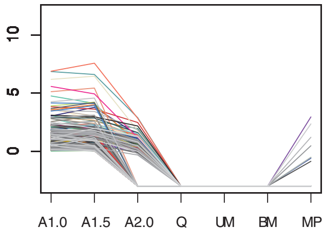
(a) Pre-meiosis/mitosis related N=234
