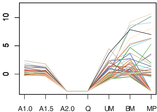
(f) Meiotic valley N=66
