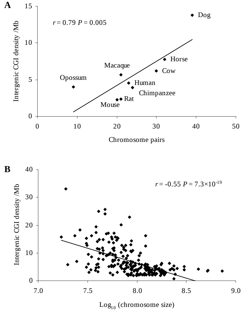
Figure S2 Correlations between Intergenic CGI density and genomic features in 9 mammalian genomes (A) Intergenic CGI density (per Mb) vs. number of chromosome pairs. (B) Intergenic CGI density (per Mb) vs. \log_{10} (chromosome size). (C) Intergenic CGI density (per Mb) vs. chromosome GC content (%). (D) Intergenic CGI density (per Mb) vs. chromosome \text{Obs}_{\text{CpG}}/\text{Exp}_{\text{CpG}} .
