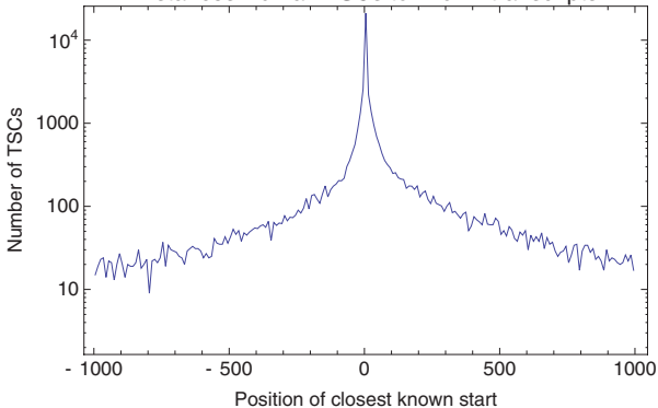
Distances Human TSCs to known transcripts
