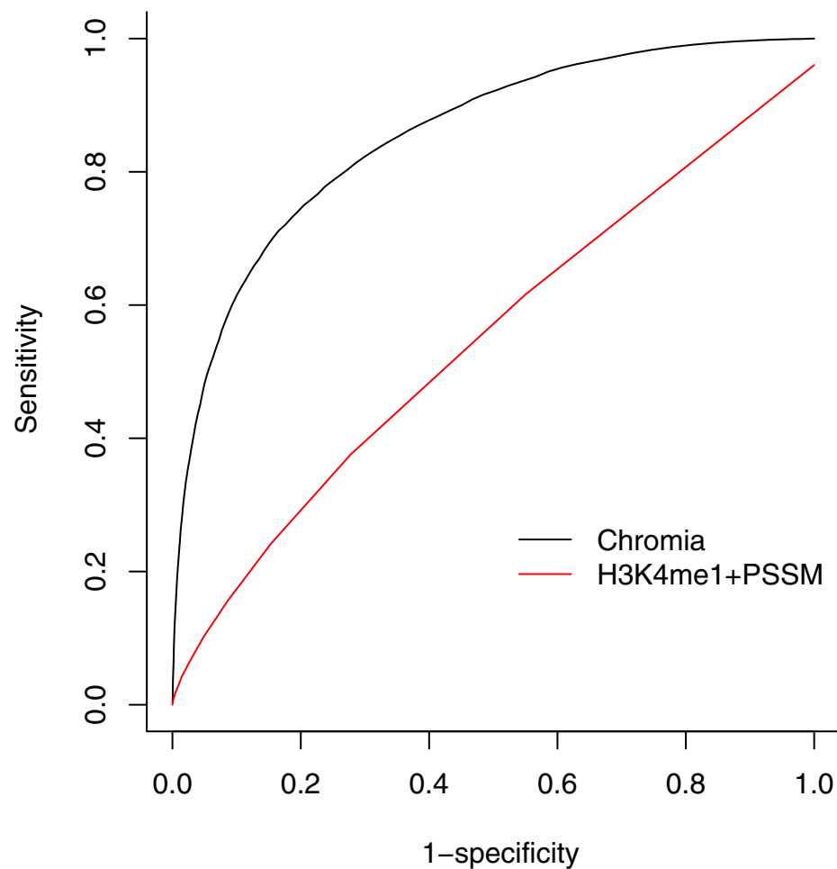
Oct4-Sox2Nanog enhancer
