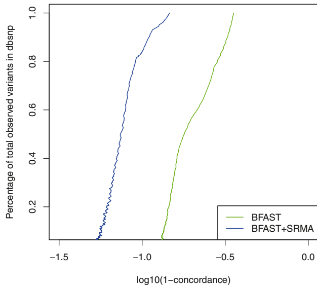
Insertions
