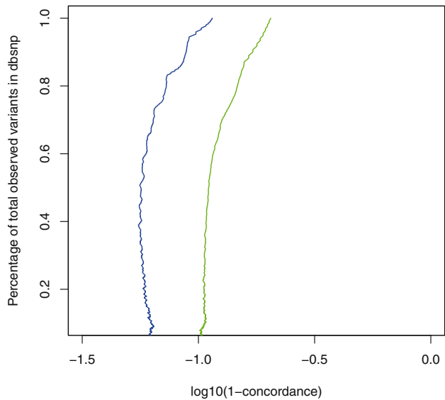
Deletions
