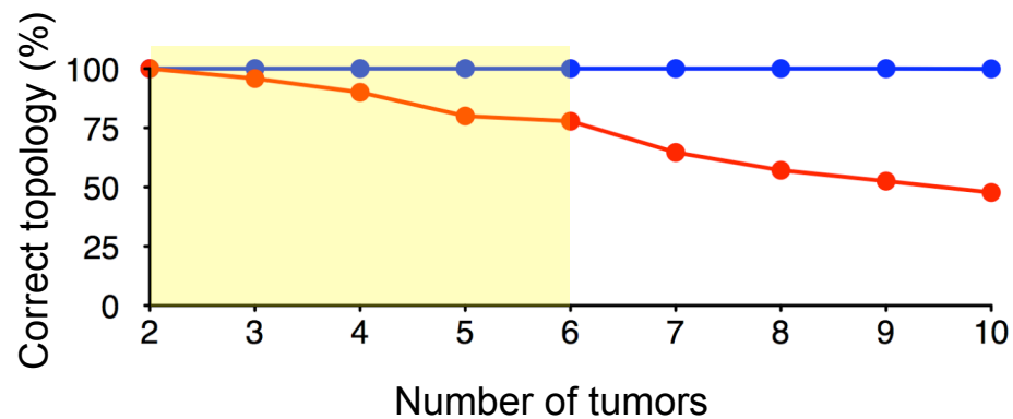
Topology of the reconstructed trees
