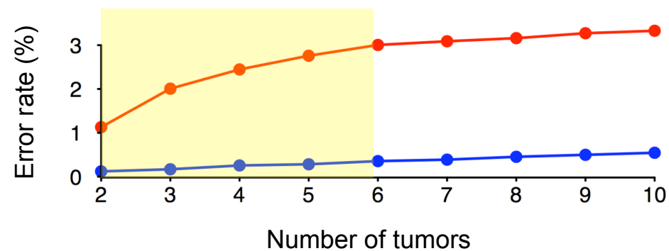
Copy number profiles of internal nodes
