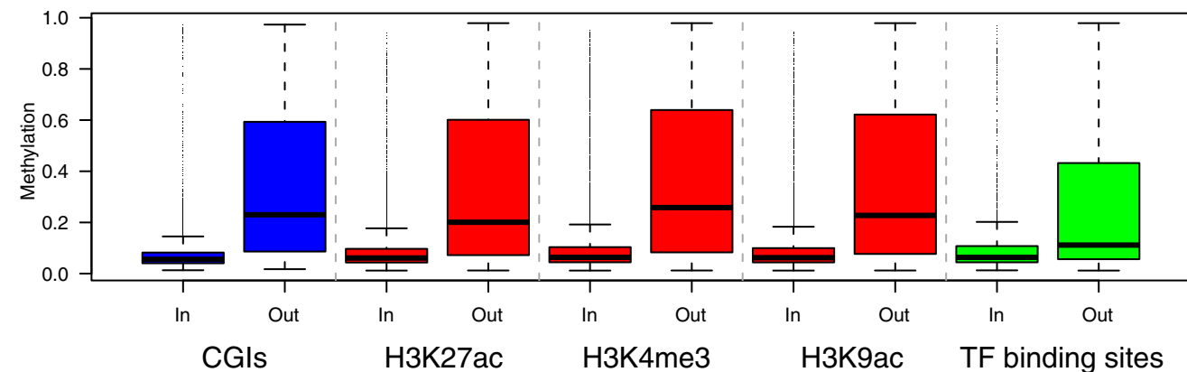
(d) Methylation in CGIs, histone modifications, and TF binding sites
