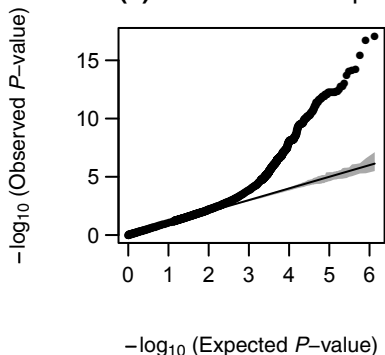
(a) cis-meQTL QQ plot
