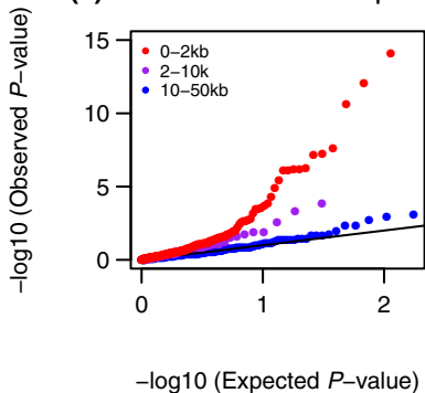
(b) meQTLs affect multiple CpGs
