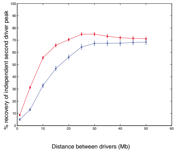
Sensitivity vs. Driver Distance
