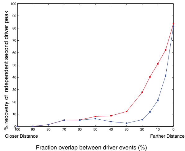
Sensitivity vs. Driver SCNA Overlap
