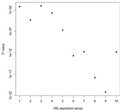
T-test p-values of exon/intron signal differences by expression group
