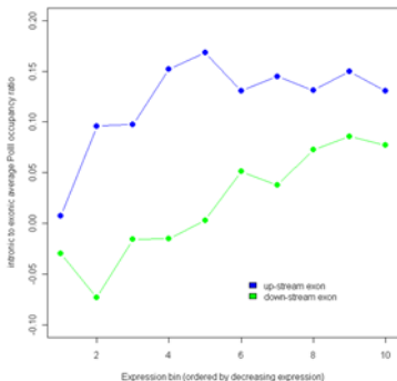
Intron:exon ratios of Pol II signal by expression bin
