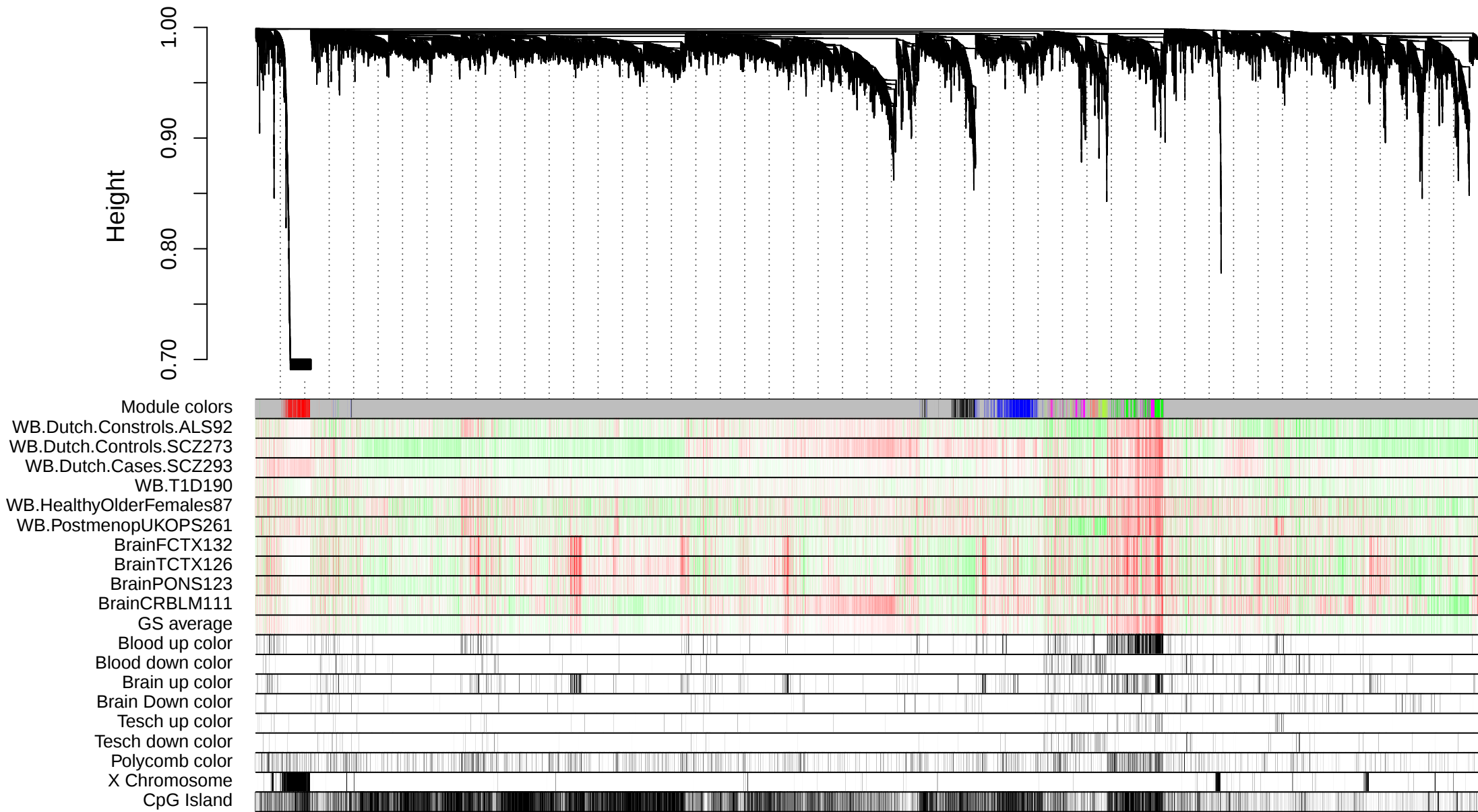
Consensus gene dendrogram and module colors for the 10 methylation dataset recut
