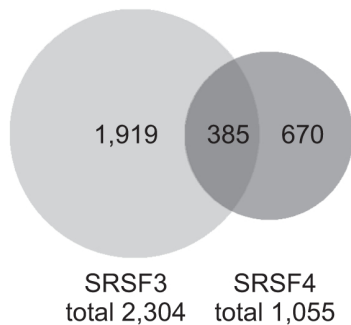
B. Genes with significant crosslink sites
