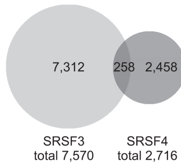
C. Significant CLIP-tag clusters
