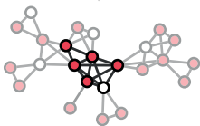
The most interconnected genes form the core SuM
