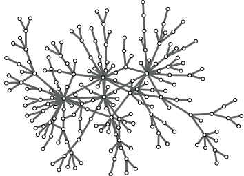
Human protein-protein interaction network
