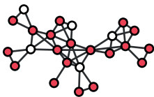
Overlapping cliques form the Suceptibility Module (SuM)
