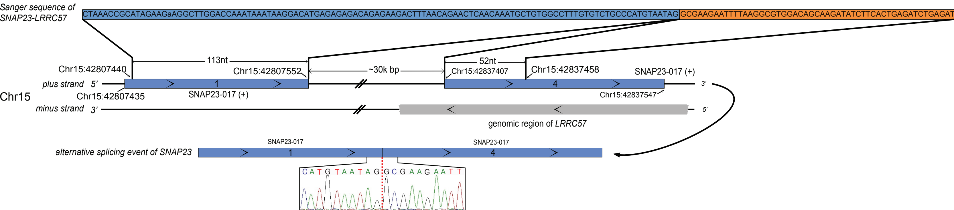
(b) SNAP23-LRRC57 analysis based on Ensembl release 69 annotation database
