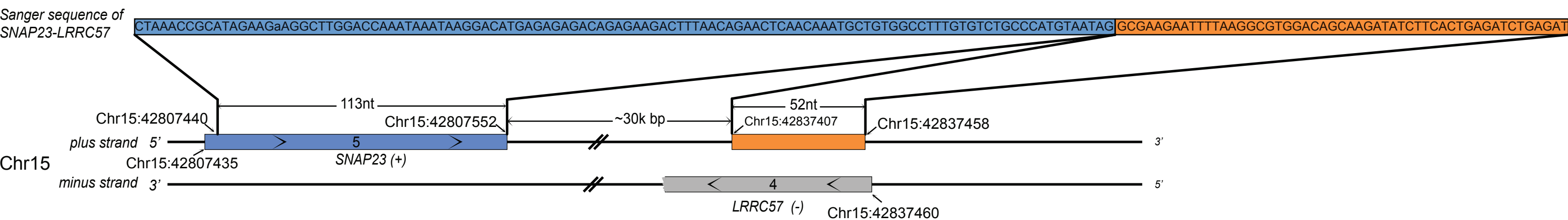
(a) SNAP23-LRRC57 analysis based on Ensembl release 59 annotation database
