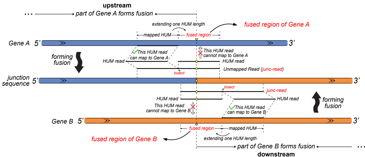
(a) getting fused regions based on unmapped reads
