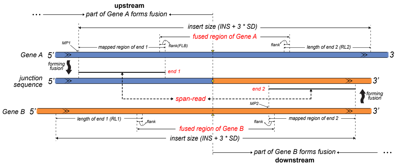
(b) getting fused regions based on span-reads
