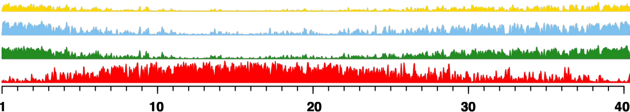
Chromosome 5
