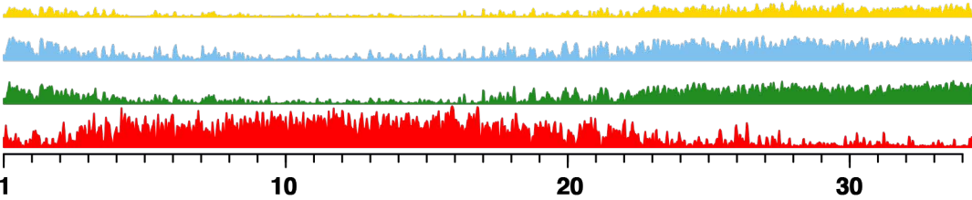
Chromosome 3
