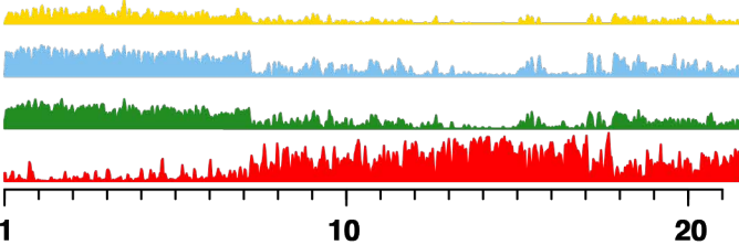
Chromosome 8
