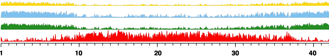
Chromosome 9
