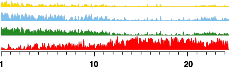
Chromosome 7
