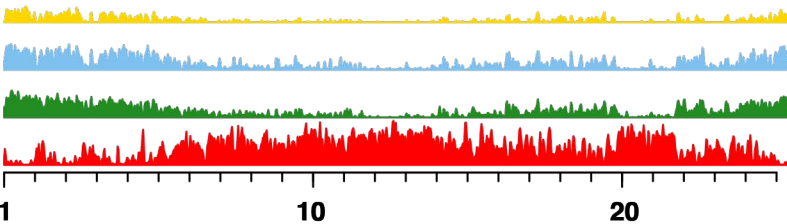
Chromosome 10
