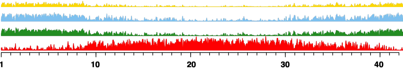
Chromosome 2
