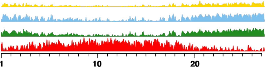
Chromosome 6
