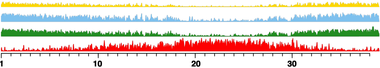
Chromosome 1
