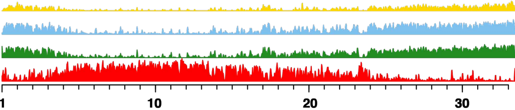
Chromosome 4
