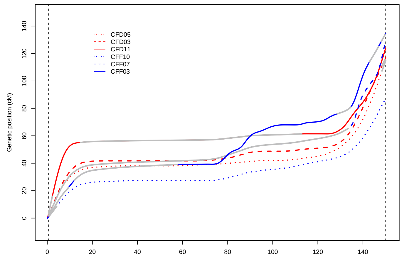
Chromosome 10
