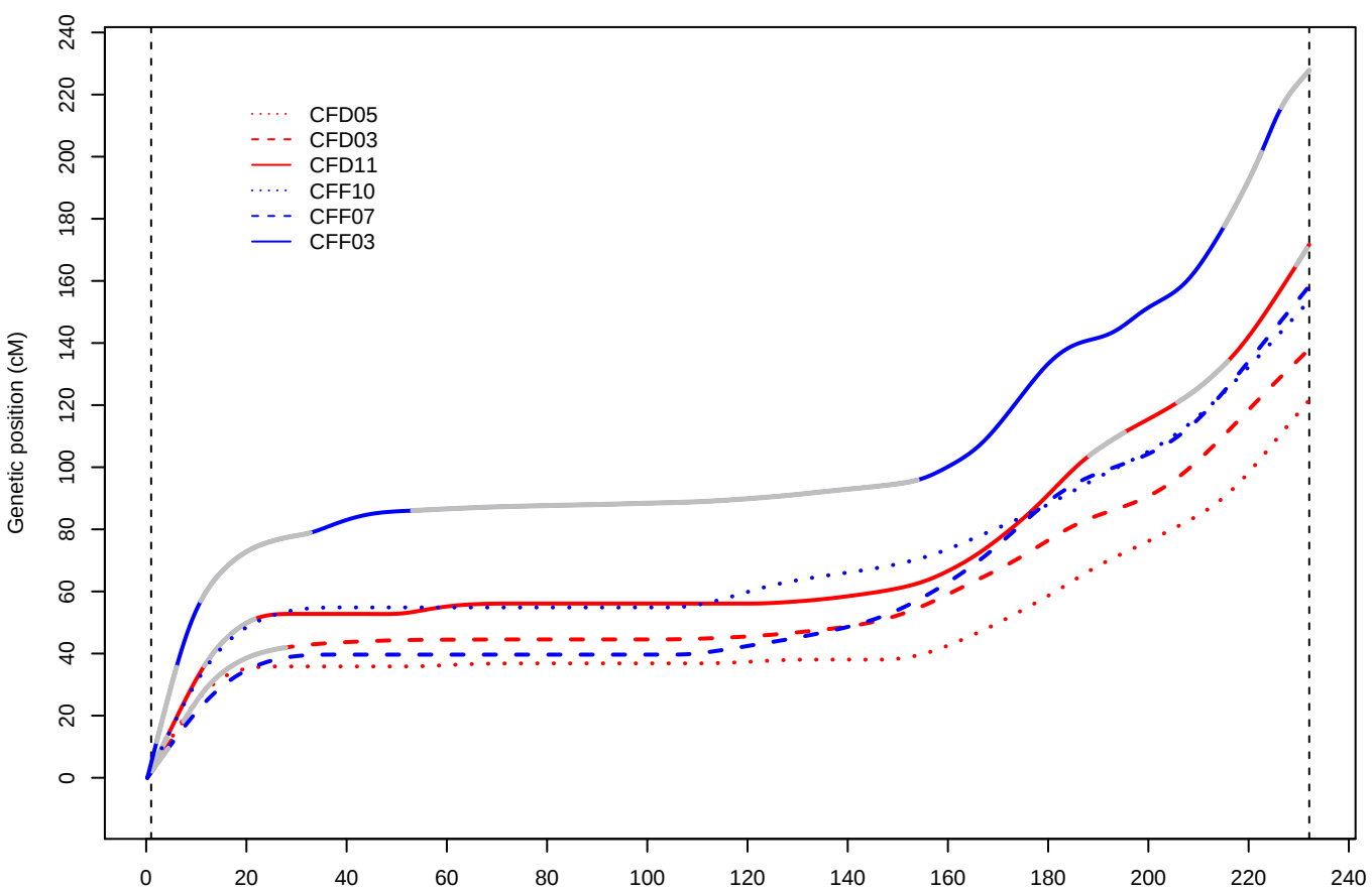
Chromosome 3
