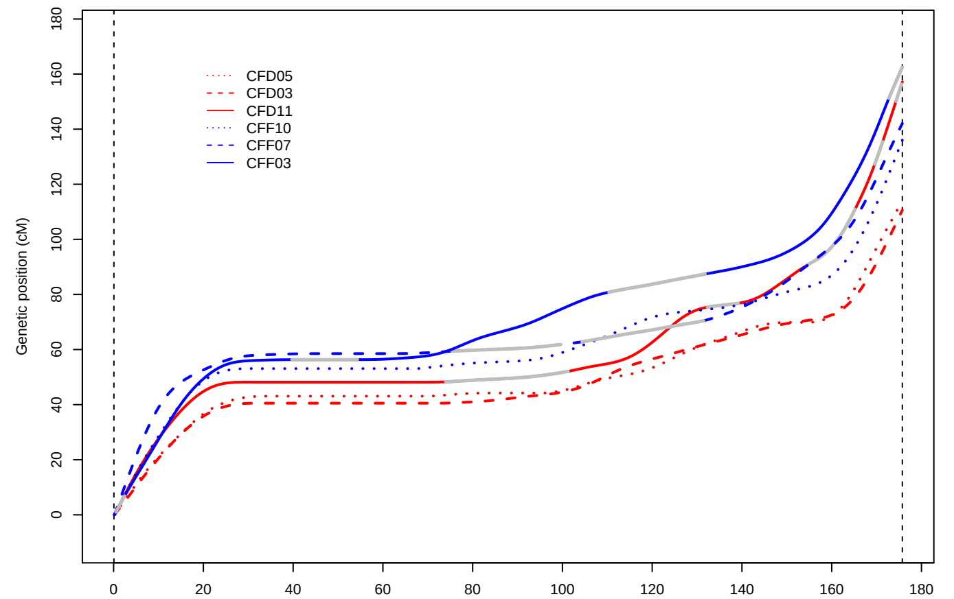
Chromosome 8
