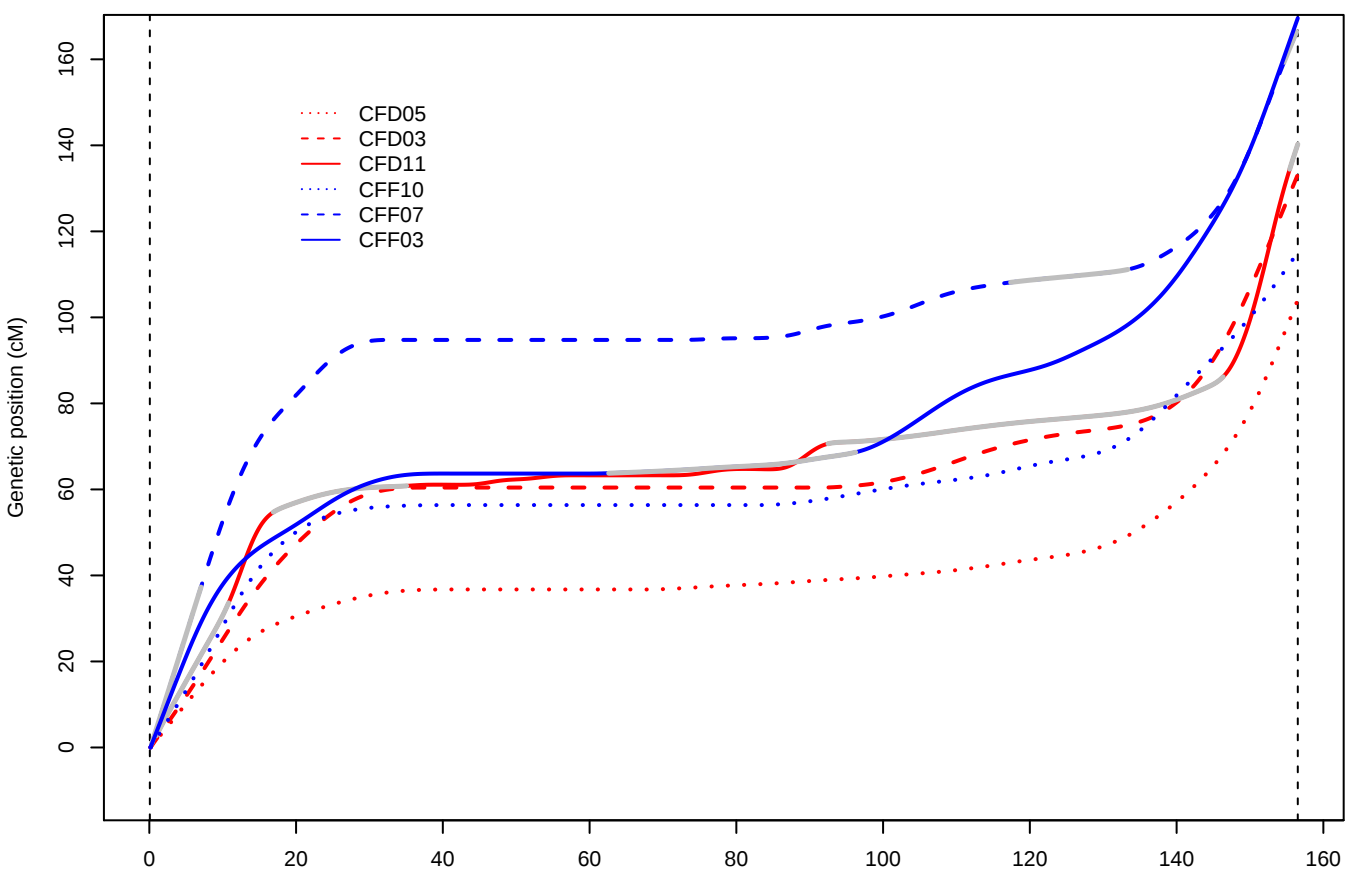
Chromosome 9
