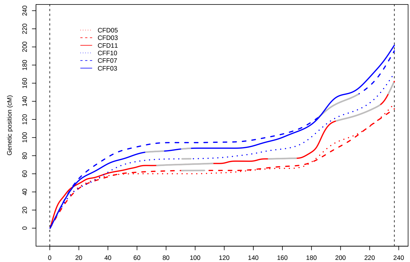
Chromosome 2
