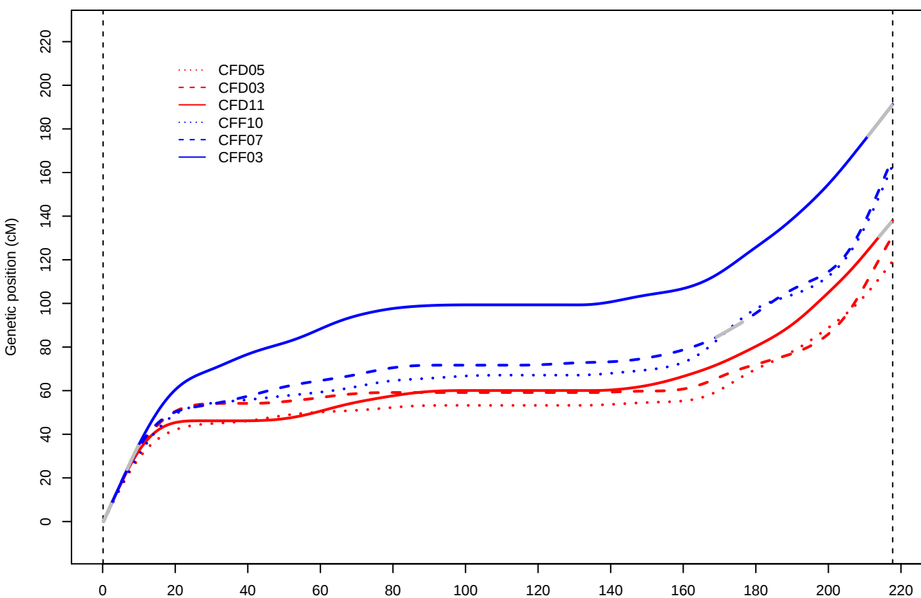
Chromosome 5
