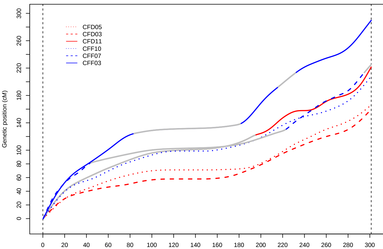
Chromosome 1
