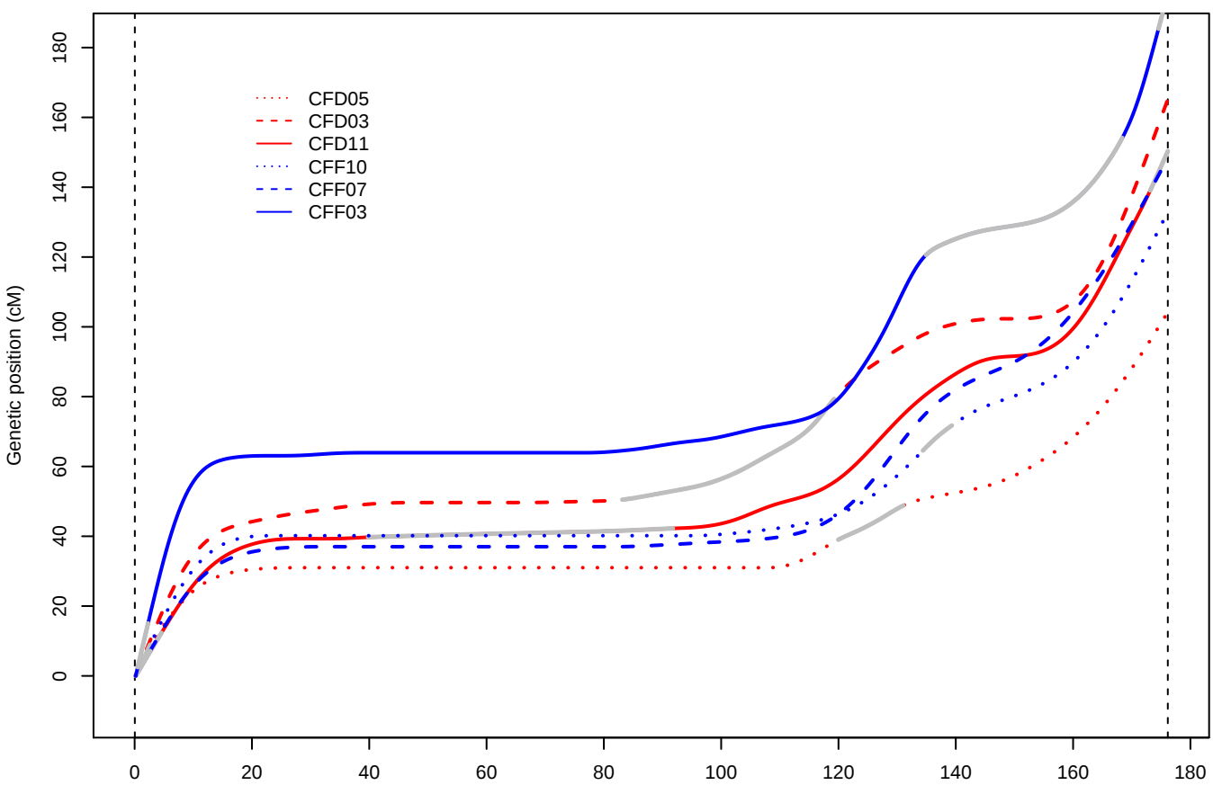
Chromosome 7
