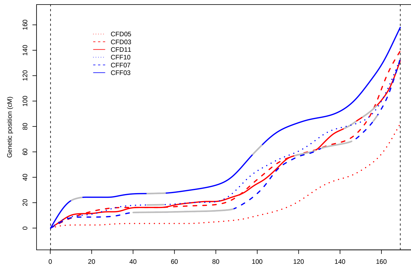
Chromosome 6
