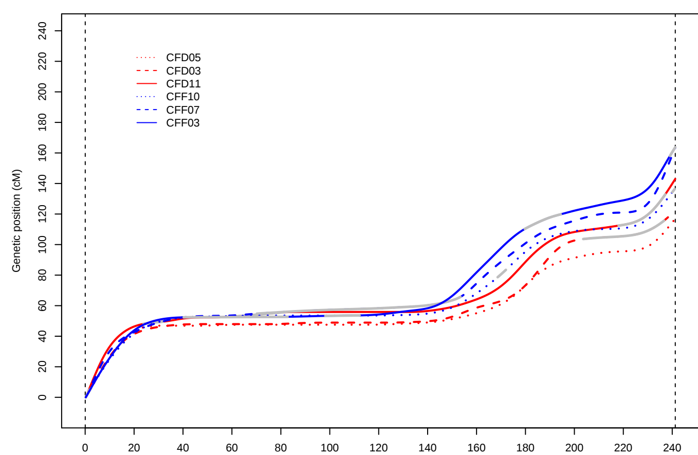
Chromosome 4
