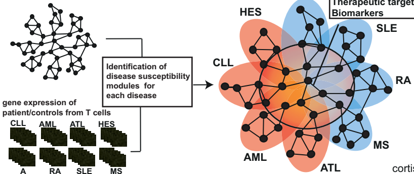
Protein-protein interaction map
