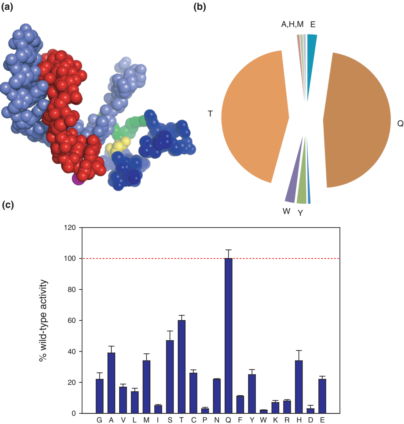
Additional data file 15. Structure, evolution and function of mjA' Q828
