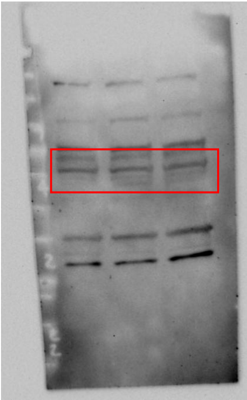
COX2
