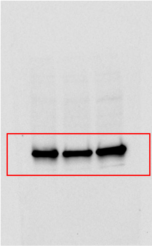
GAPDH
