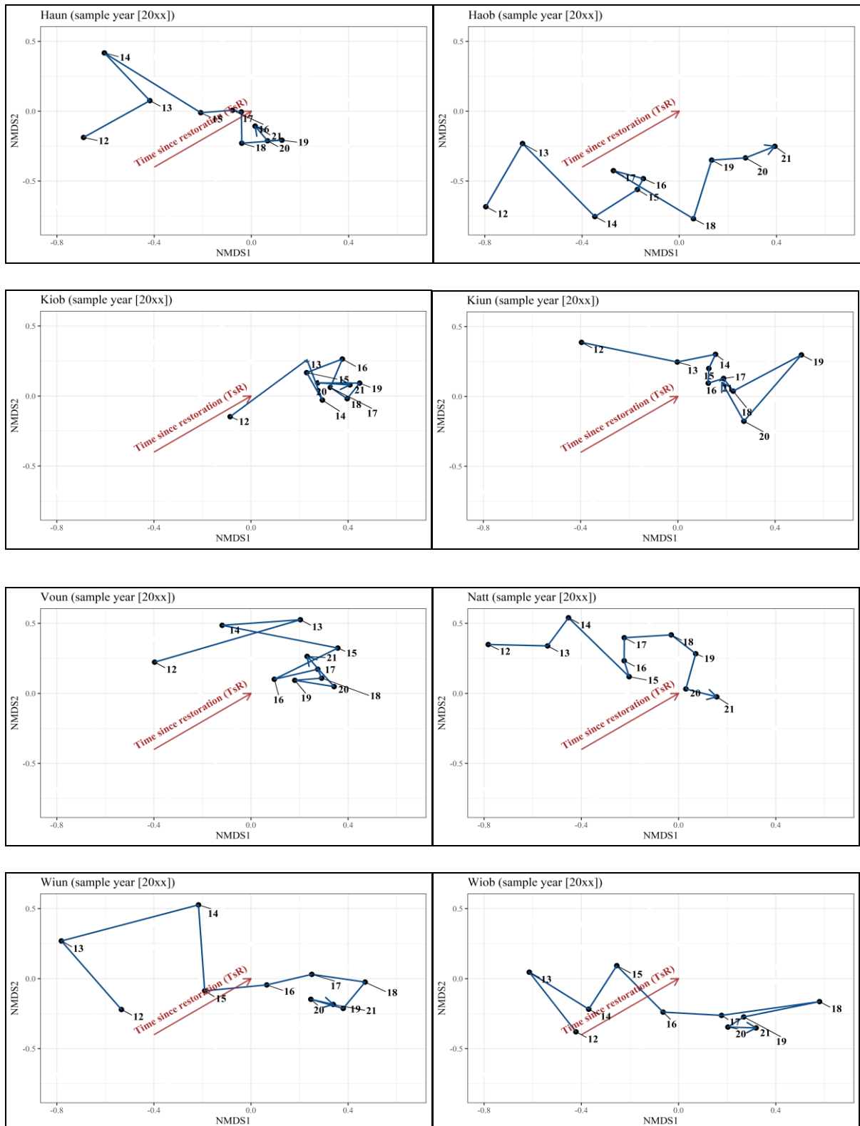
Figure S1. NMDS of log-transformed community data per sampling site, sampling years connected. Time since restoration was added as an overlay (red arrow).
