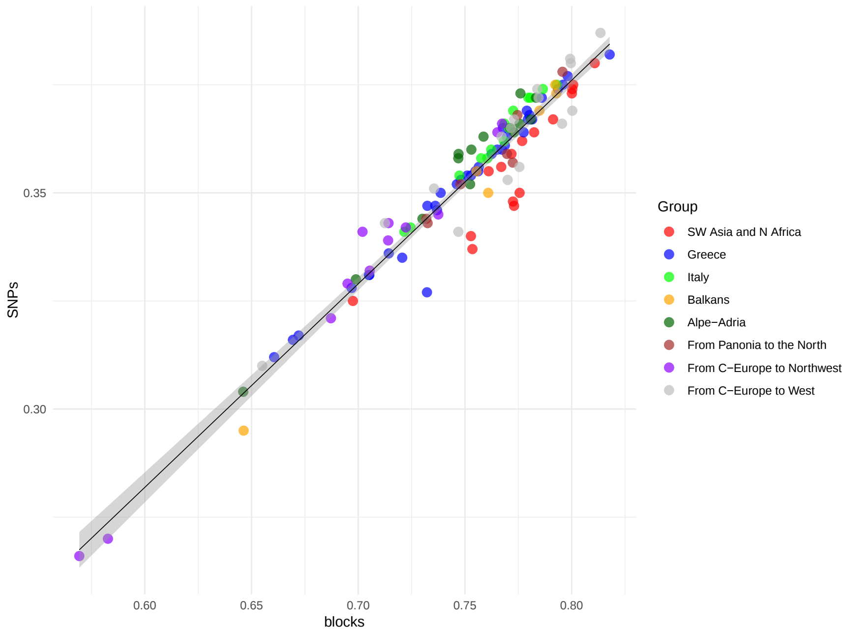
Scatter Plot of H_o _(blocks) vs H_o _(SNPs)
