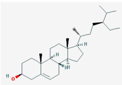
B-sitosterol
