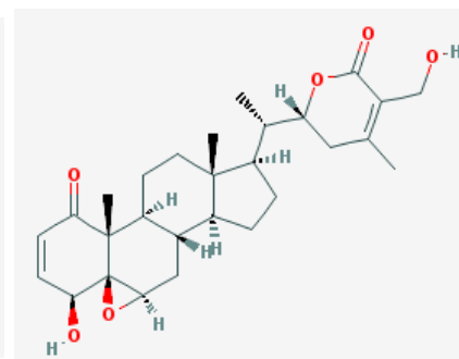
Withanerin A
