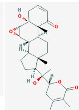
Withanolide A
