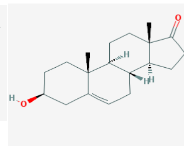
Dehydro epiandrosteron
