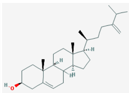
24-methylene cholesterol
