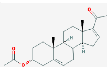
16-DPA
