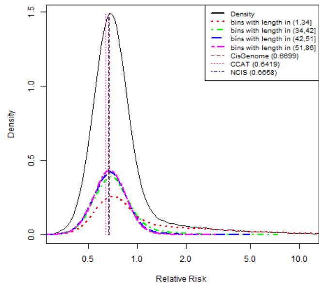
(b) CTCF, K = 100
