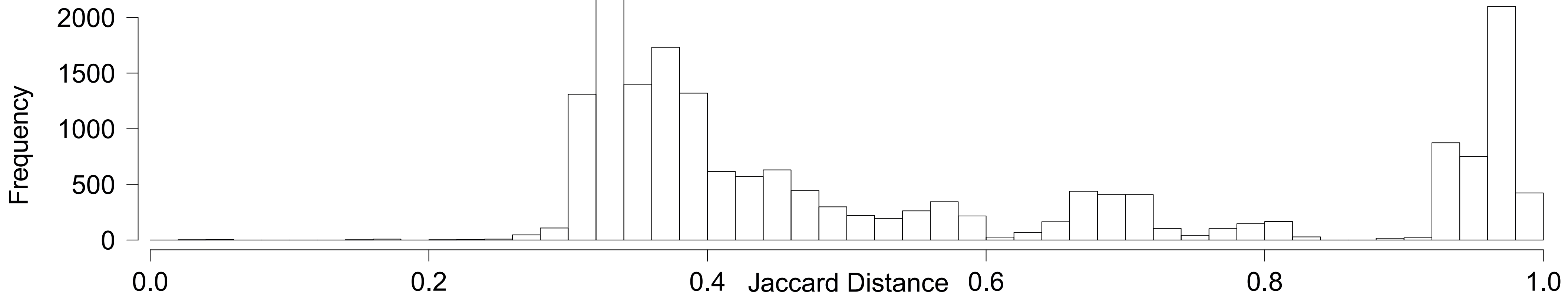
17-mer
