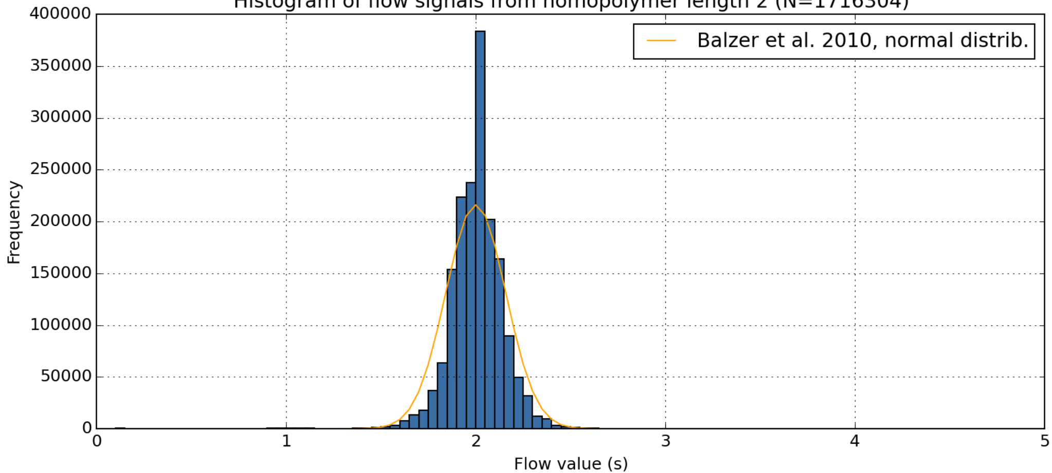
Histogram of flow signals from homopolymer length 2 (N=1716304)
