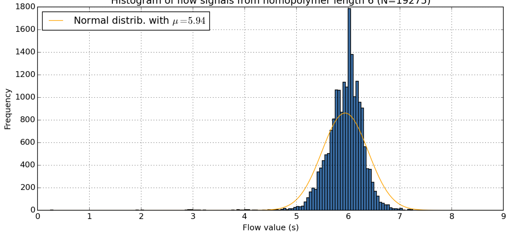
Histogram of flow signals from homopolymer length 6 (N=19275)
