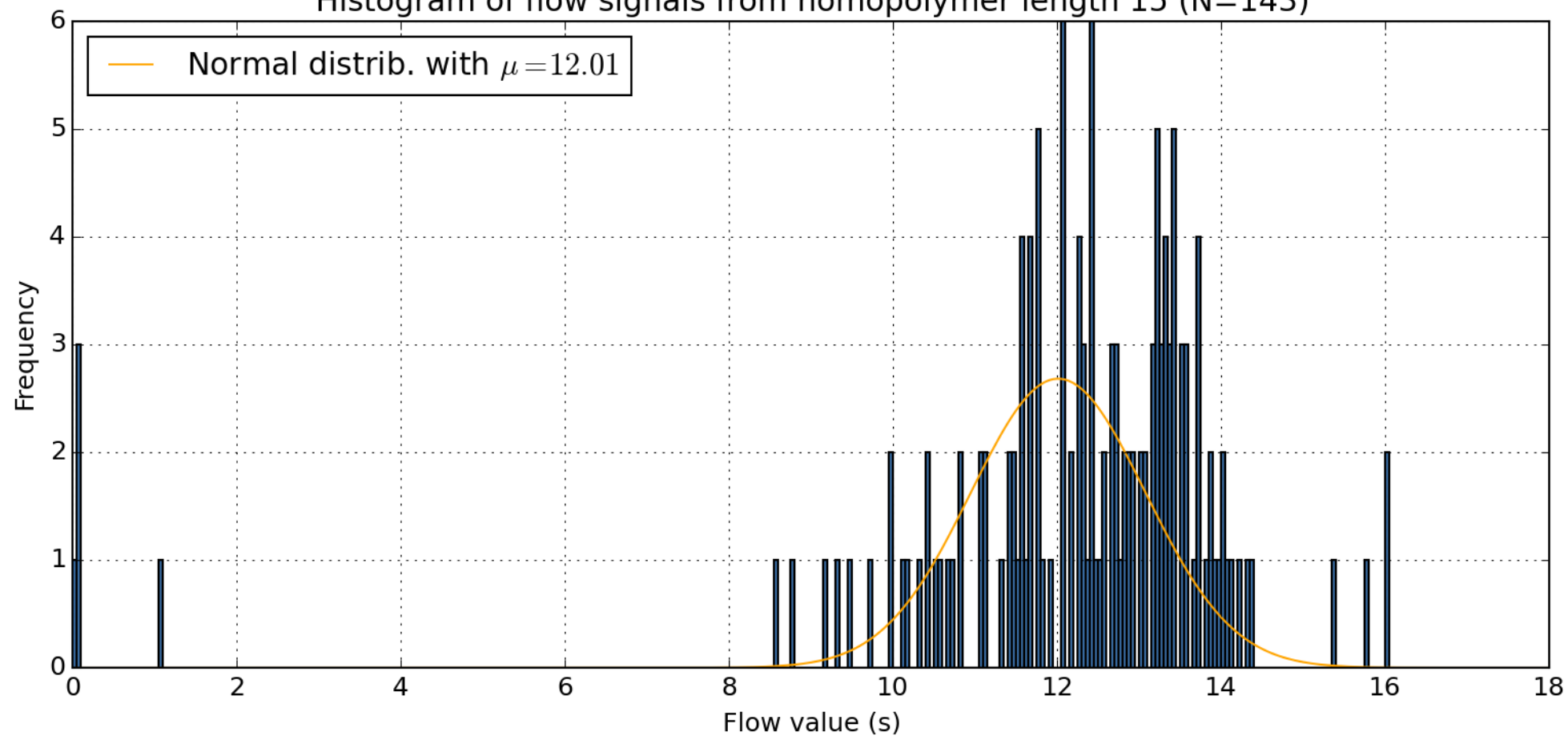
Histogram of flow signals from homopolymer length 15 (N=143)
