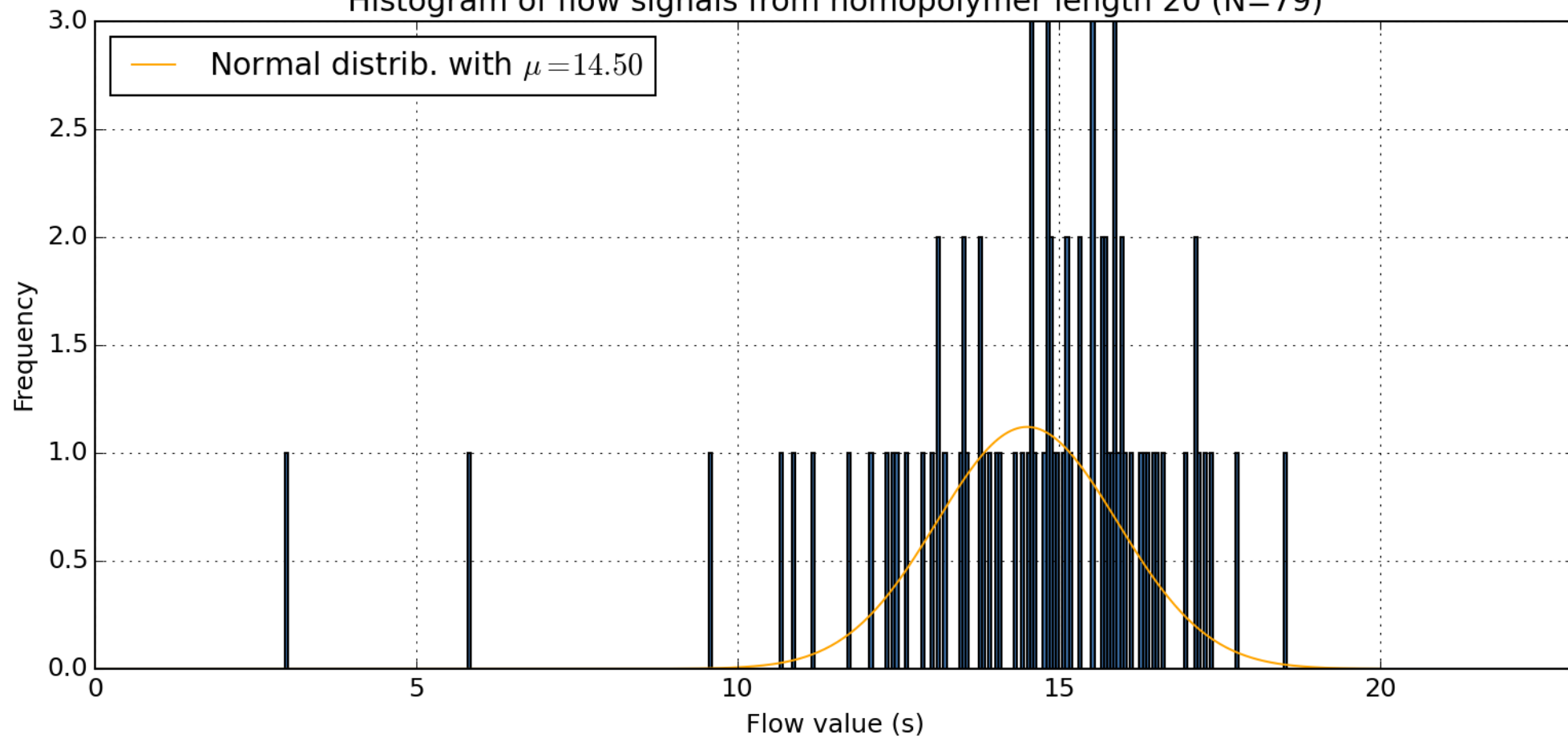
Histogram of flow signals from homopolymer length 20 (N=79)
