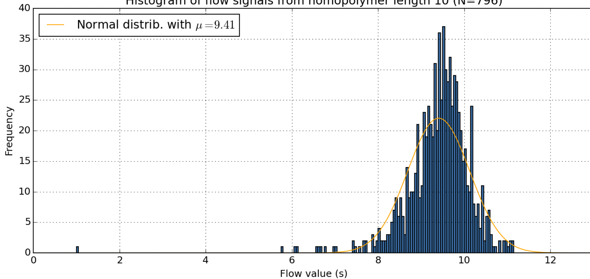
Histogram of flow signals from homopolymer length 10 (N=796)
