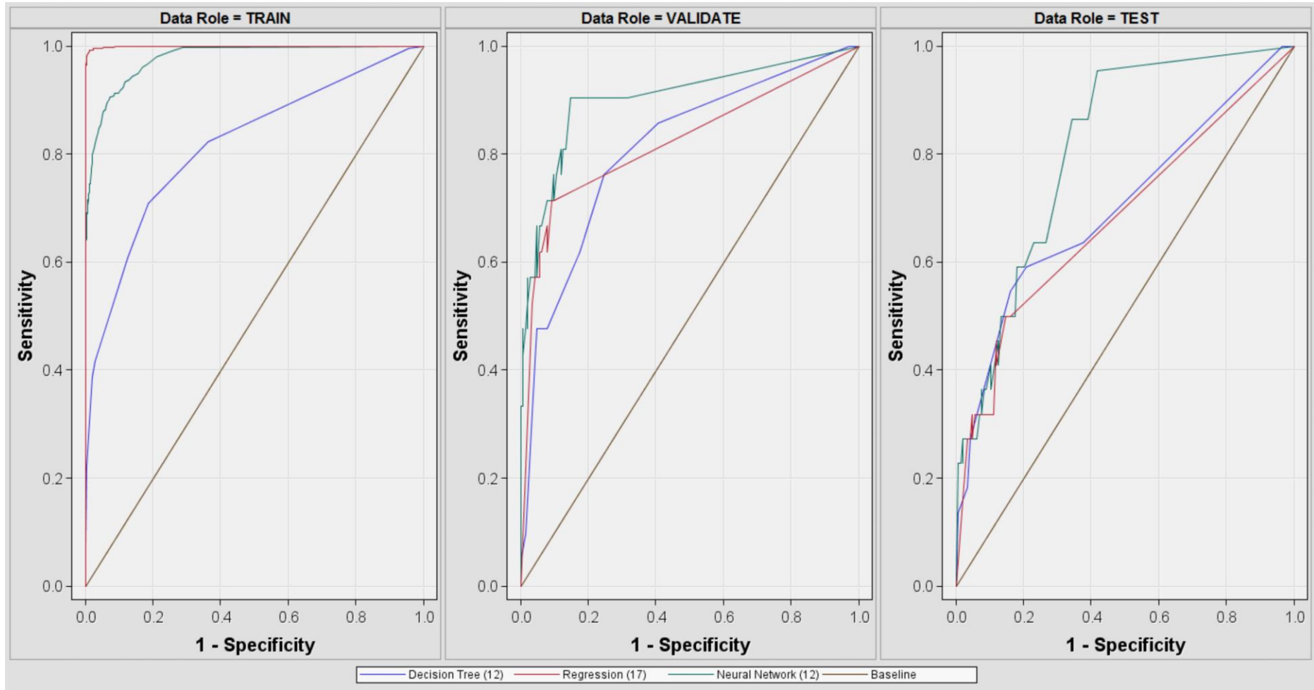
Figure S3. The ROC plots of training, validation, and test sets for the Schilling dataset.
