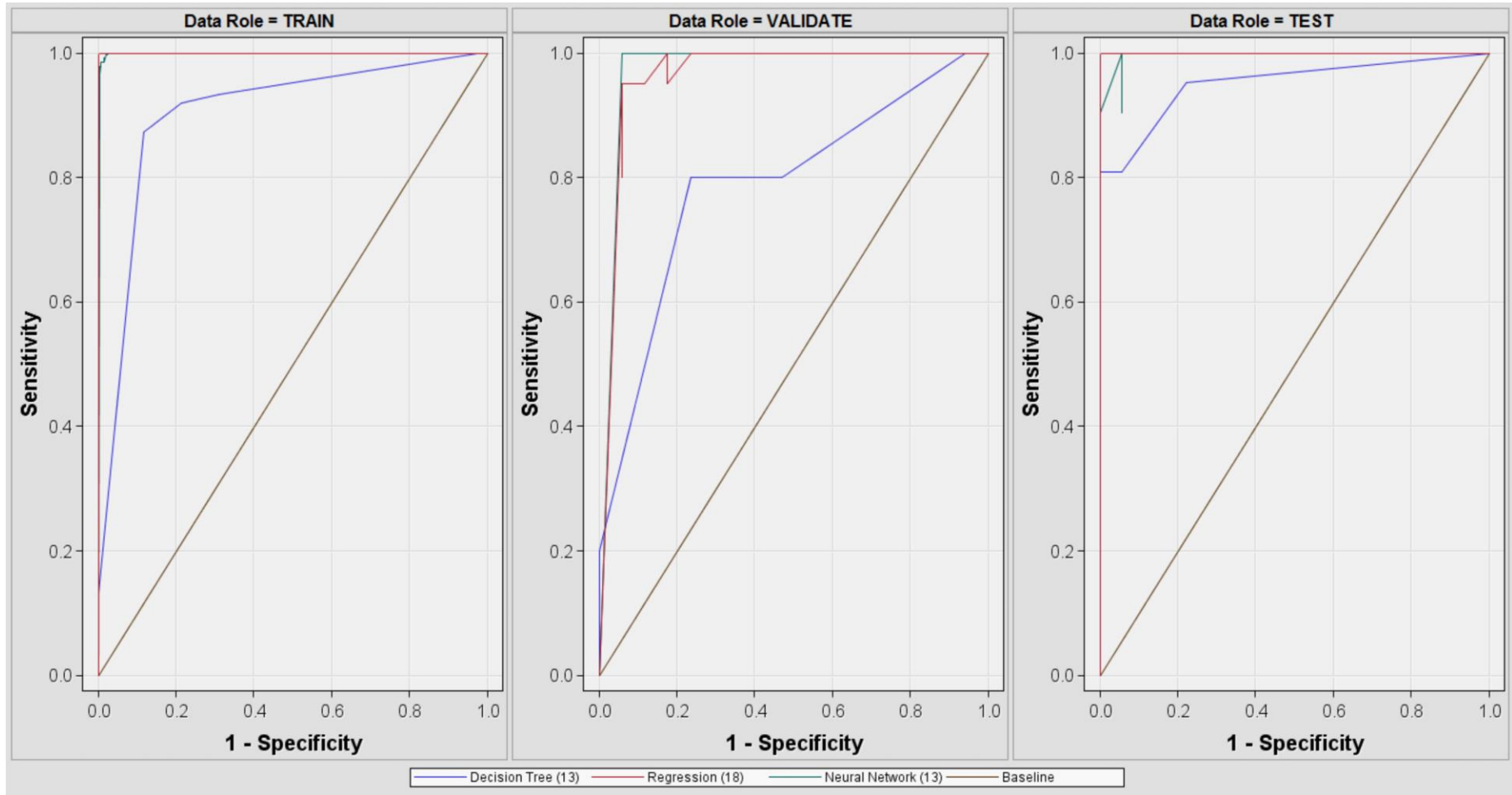
Figure S1. The ROC plots of training, validation, and test sets for the 746 dataset.
