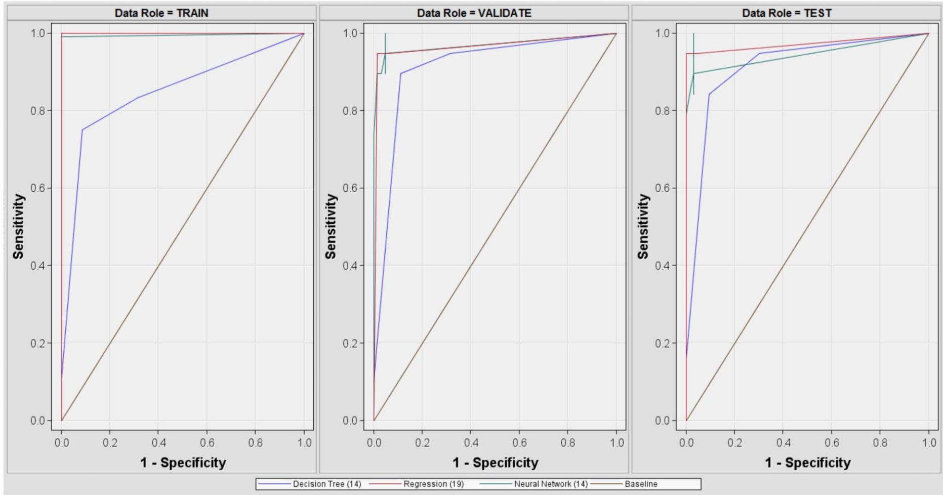
Figure S2. The ROC plots of training, validation, and test sets for the 1625 dataset.
