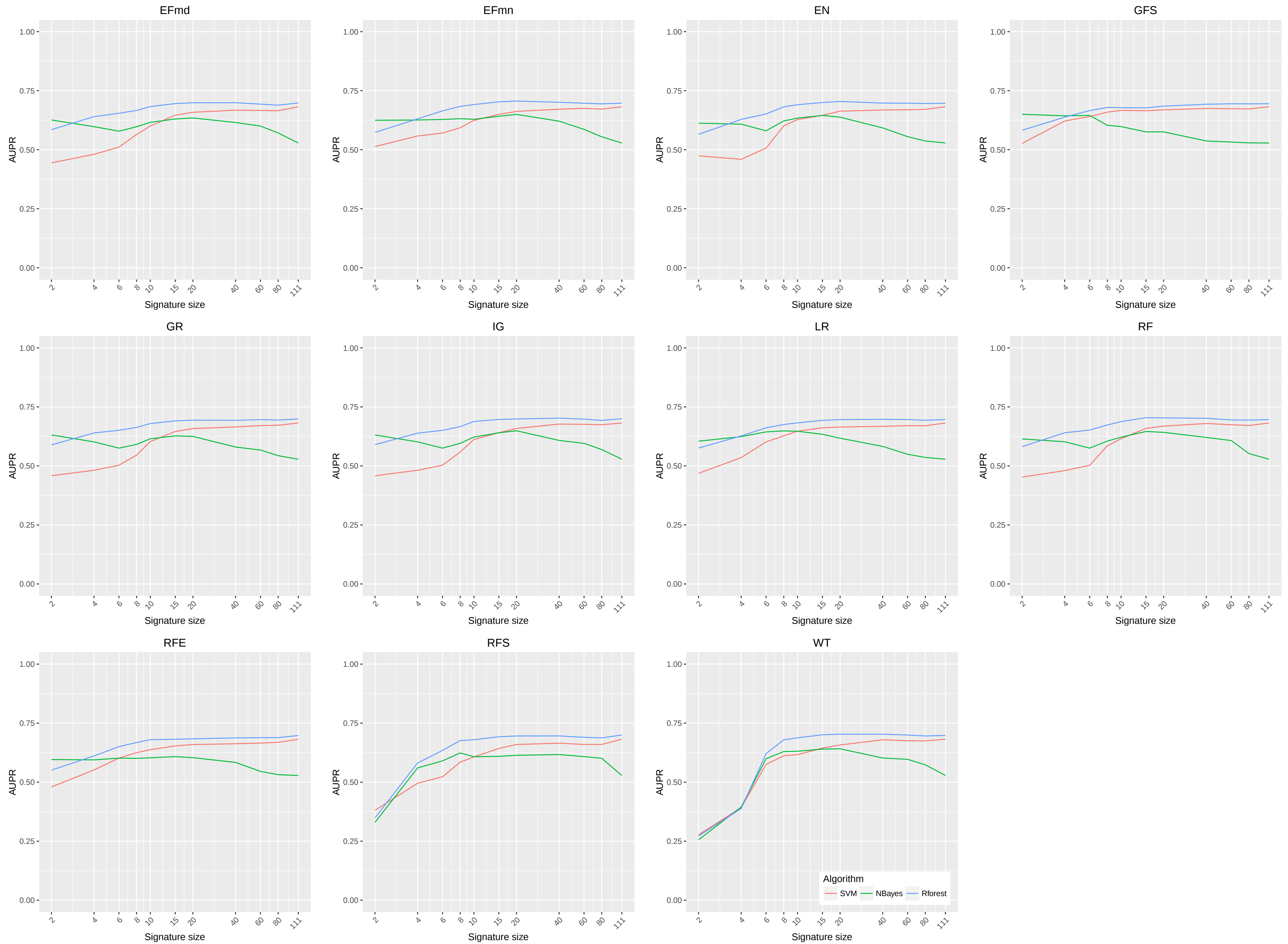
Figure S1. Prediction accuracy with different feature selection algorithms in human (10-fold average AUPR on the y-axis, signature size on the x-axis)
