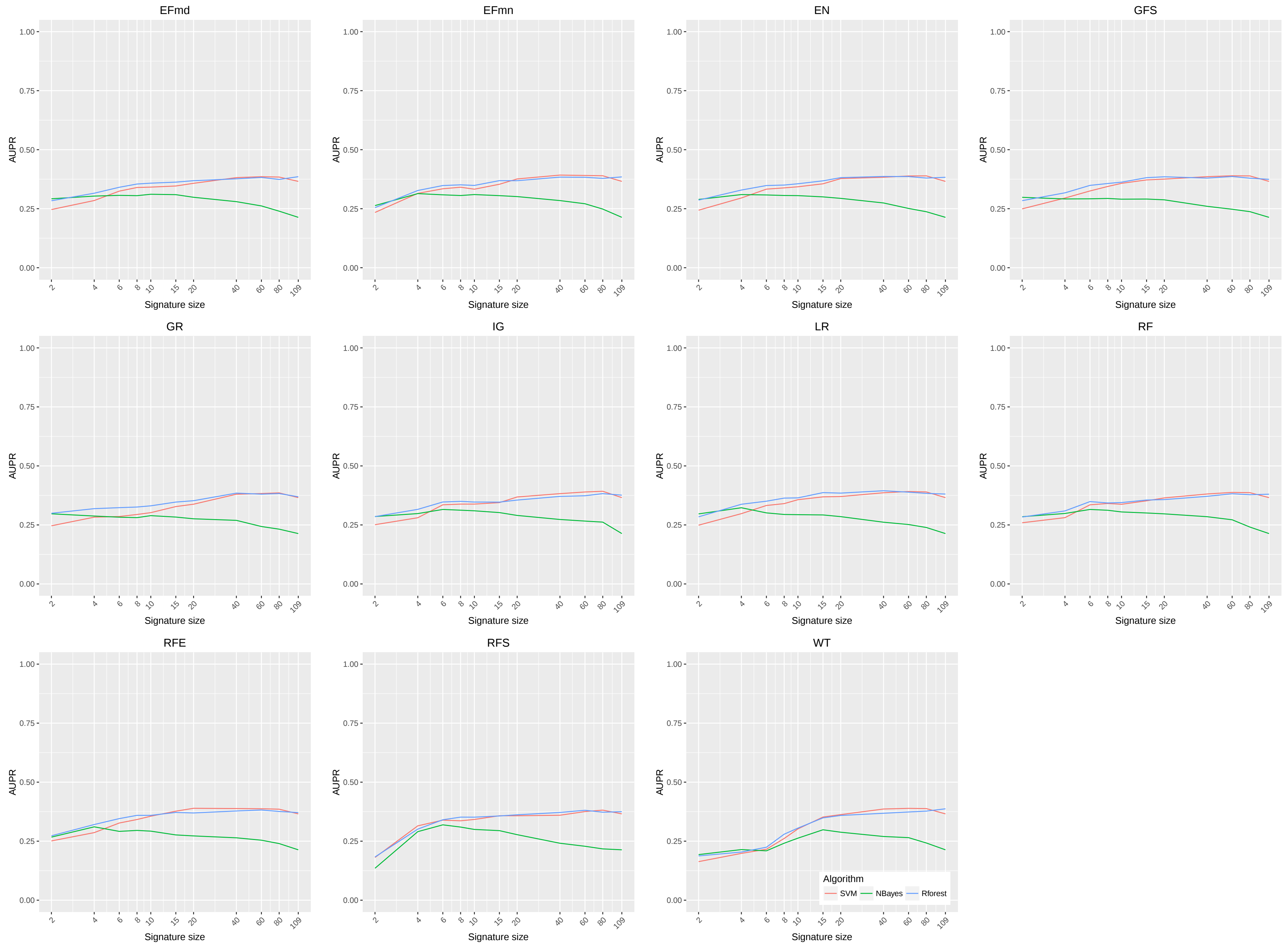
Figure S3. Prediction accuracy with different feature selection algorithms in zebrafish (10-fold average AUPR on the y-axis, signature size on the x-axis)
